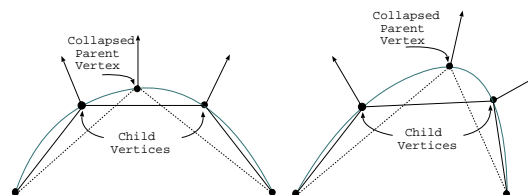
Figure 8: Effect of normals on the position of the collapsed vertex
