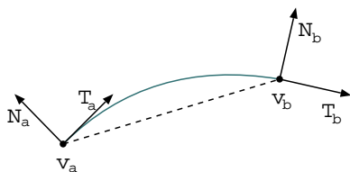
Figure 6: Hermite Cubic Curve
