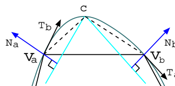
Figure 7: Computing the position of the collapsed vertex
