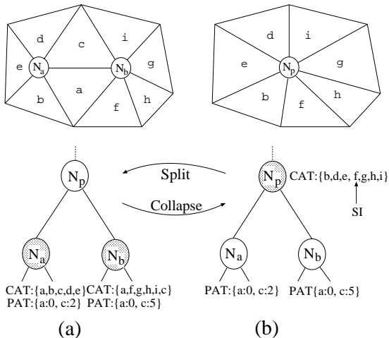
Figure 2: Adjacent triangle update after split and collapse
