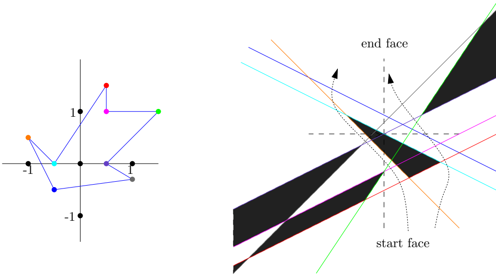
Figure 7: A simple polygon and the dual arrangement of its vertices. Forbidden faces are gray; two valid paths—through white faces only—are shown
