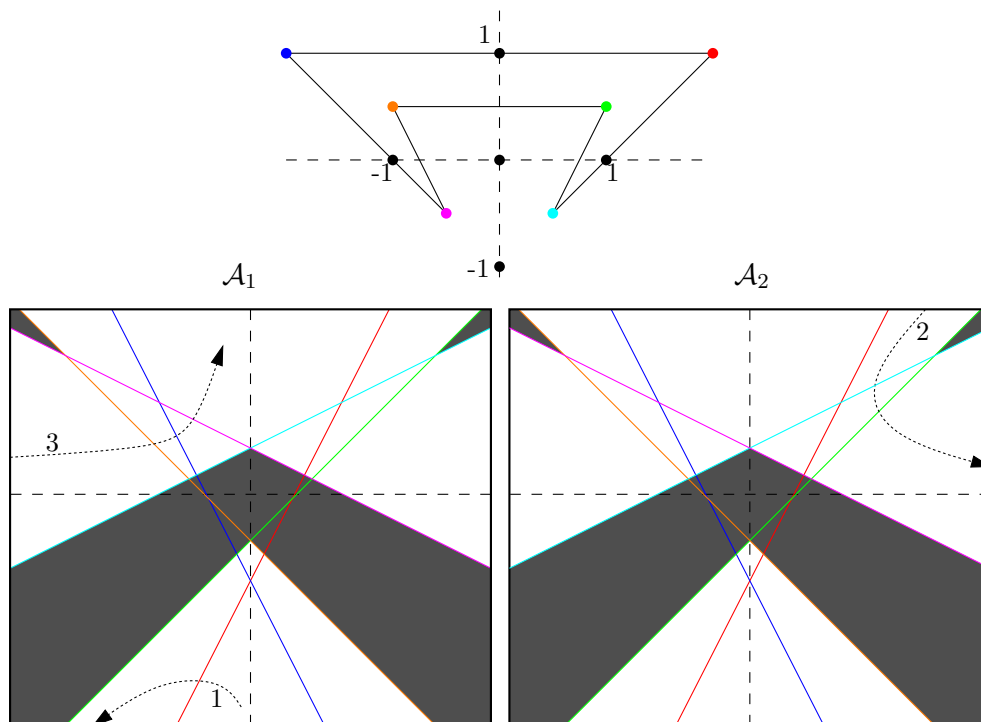
Figure 8: A simple polygon and the dual arrangements \mathcal{A}_1 and \mathcal{A}_2 . Any valid sweep over the polygon (for example, the one shown by the arrows 1, 2, 3) must go via faces of both arrangements.
