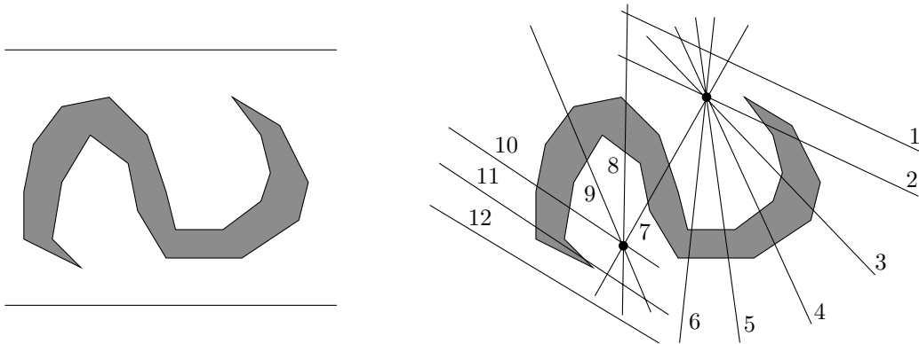
Figure 5: The top line shows the position before the sweep; the bottom line after the sweep. Several possible intermediate positions are shown in the figure on the right.
