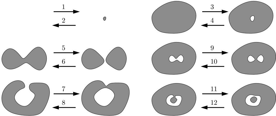
Figure 2: Topological changes that can occur in the cross-sections.
