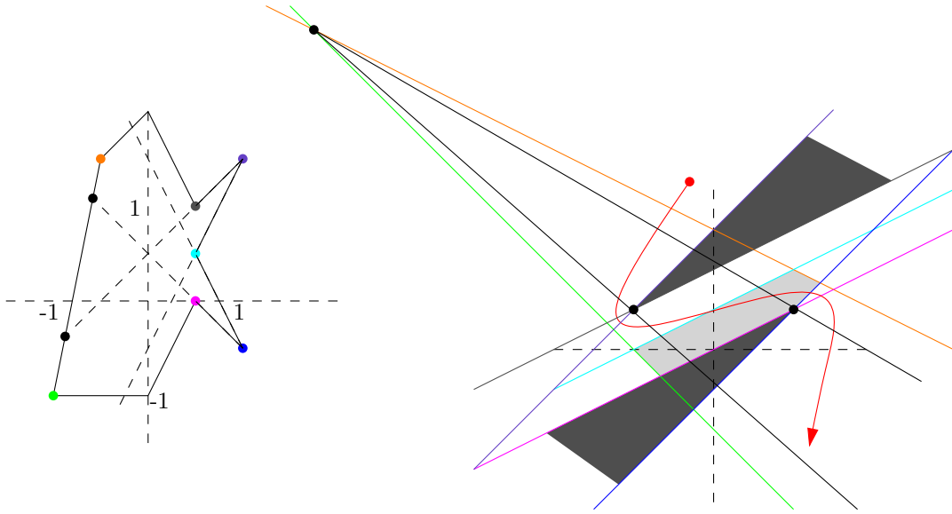
Figure 10: The example of Figure 9 with the extensions in primal and dual shown.
