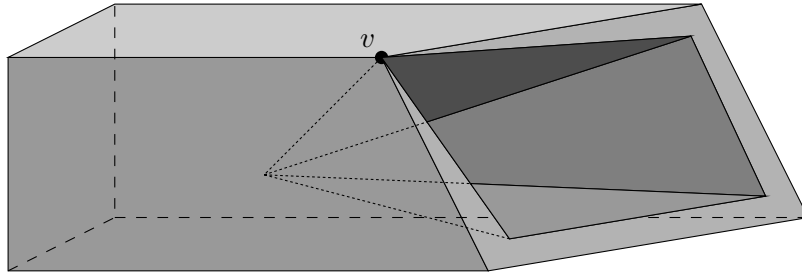
Figure 4: A close-up view of the vertex in Figure 3.
