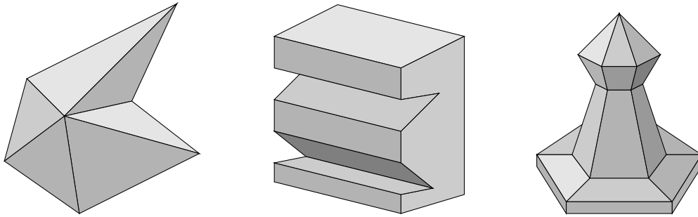
Figure 1: Polyhedra with convex cross-sections only.
