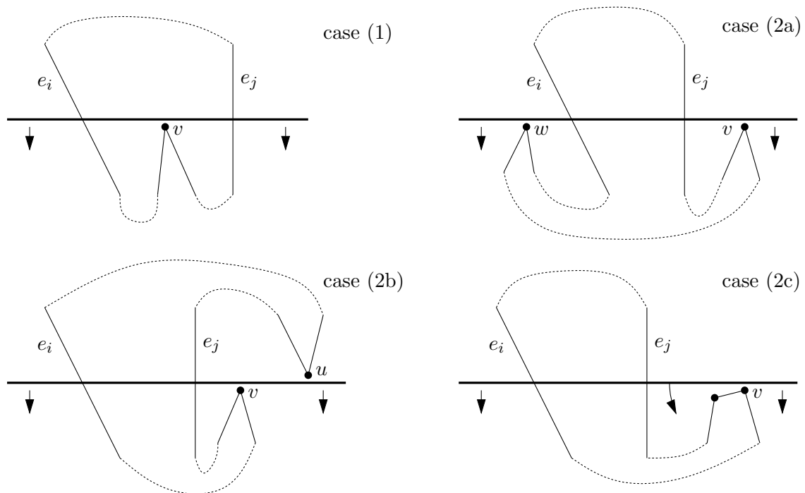
Figure 11: Illustration of the proof.
