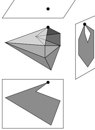
Figure 3: A vertex that causes different types of topological change for different sweep directions
