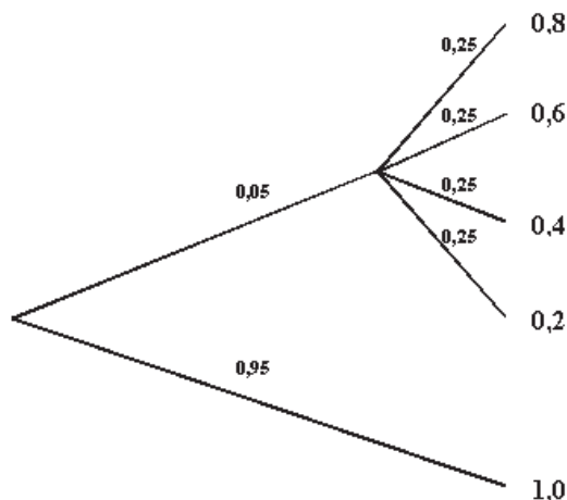
Fig. 1. Graphical representation of expected loss calculation assuming independence between default probability and severity.
