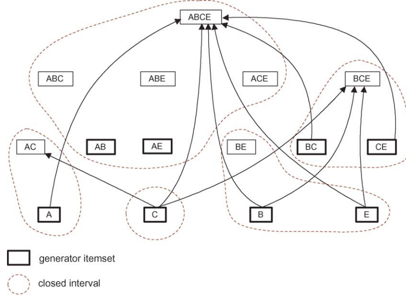
Figure 11. Approximate min-max association rules extracted from \mathcal{D} .
