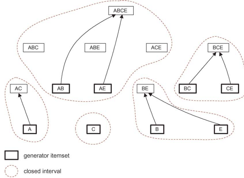
Figure 8. Exact min-max association rules extracted from \mathcal{D} .
