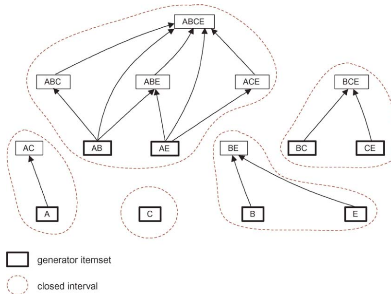
Figure 7. Exact association rules extracted from \mathcal{D} .
