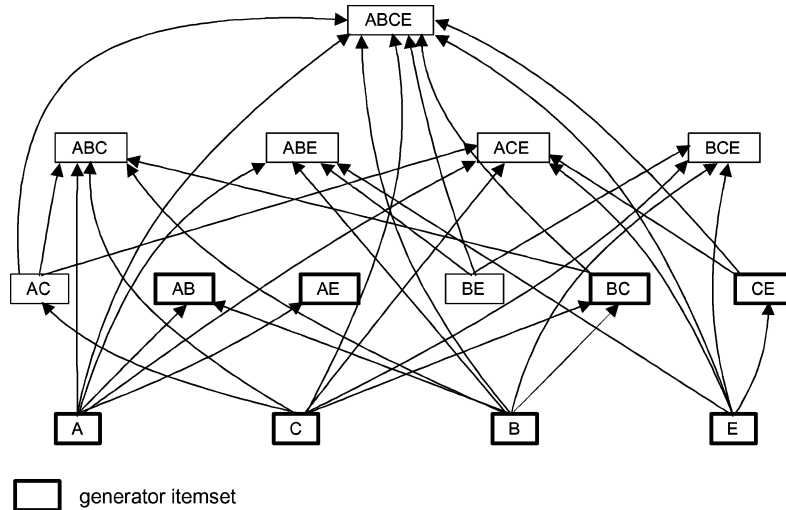
Figure 10. Approximate association rules extracted from \mathcal{D} .
