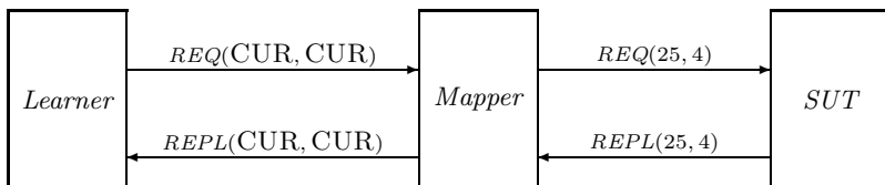
Fig. 2. Introduction of Mapper module
