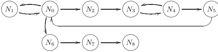
FIGURE 5. Graph of the Network \mathcal{N} used in the proof of Theorem 3.1.
