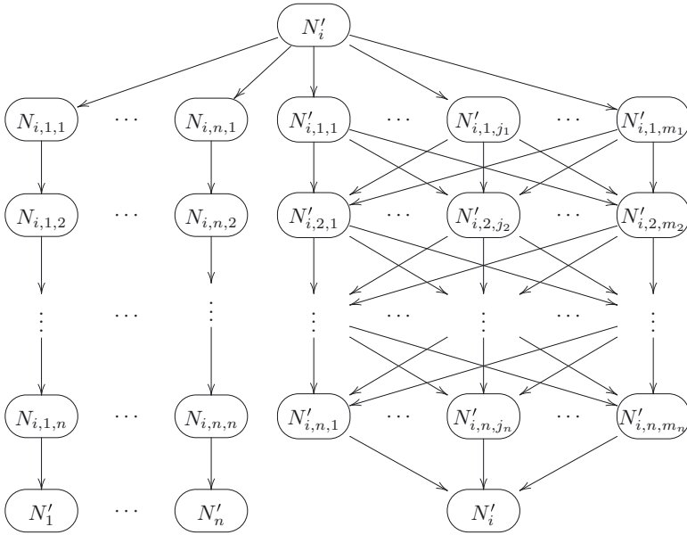
FIGURE 3. Graph of the subnetwork s(N_i) , defined in the Proof of Theorem 2.1.
