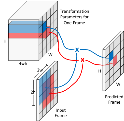
Figure 3: Transformations: For each (x, y, t) coordinate in the future, the network estimates a weighted combination of neighboring pixels from the input frame to render the predicted frame. The \times denotes dot product. Note the transformation is applied by convolution.
