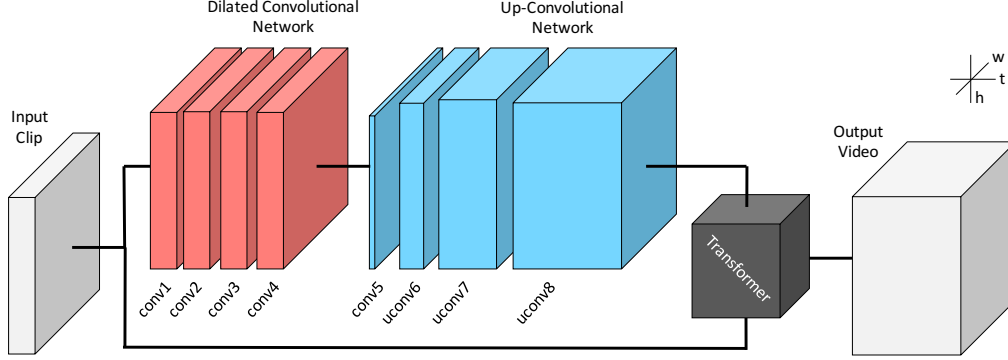
Figure 4: Network Architecture: We illustrate our convolutional network architecture for generating the future. The input clip goes through a series convolutions and nonlinearities that preserve resolution. After integrating information across multiple input frames (if multiple), the network up-samples temporally into the future. The network outputs codes for a transformation of the input frames, which produces the final video. For details on the transformer, see Figure 3.
