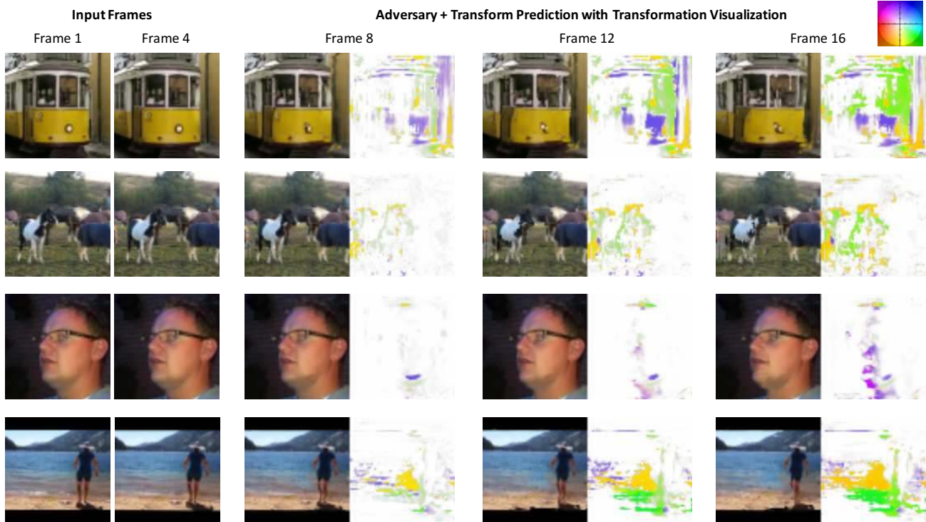
Figure 7: Visualizing Inferred Transformation: We visualize the transformation generated by our full model. Colors indicate direction that pixels move relative to the input frame under the transformation. The model learns to mix neighboring pixels of the input to generate the future frames.
