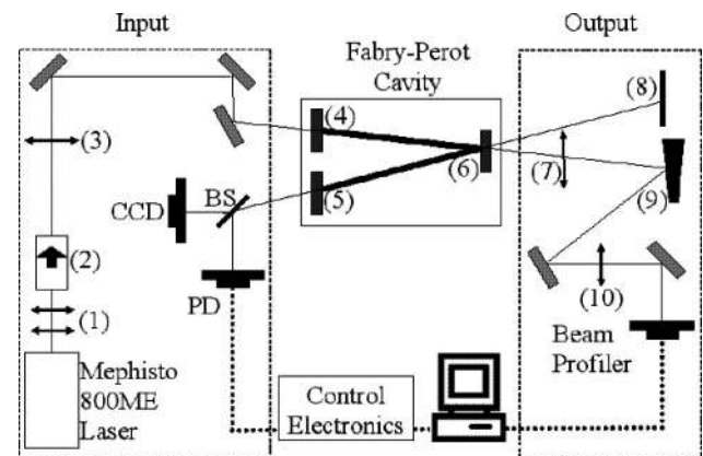
Fig. 3. Schematic of the mesa beam cavity prototype experimental setup: the two optical benches, the cavity tank, the control electronics, and the profile acquisition. Solid lines denote optical signals; dotted lines denote electronic signals. (1) Lenses to eliminate astigmatism, (2) Faraday isolator, (3) mode matching lens, (4) flat input mirror, (5) MH mirror, (6) flat folding mirror, (7,10) beam imaging lenses, (8) beam dump, and (9) wedged attenuating pickoff mirror. Unlabeled items are beam-steering mirrors.
