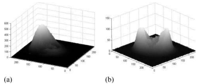
Fig. 5. Alignment of the fundamental mesa beam with astigmatic flat cavity mirrors: (a) stable, asymmetric single peak, (b) highly sensitive double peak distribution.
