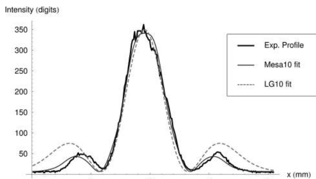
Fig. 9. Mesa TEM_{10} profile (thick black curve). The light gray curve shows the theoretical mesa TEM_{10} , which better fits the data than a Laguerre–Gauss TEM_{10} mode (dashed curve).
