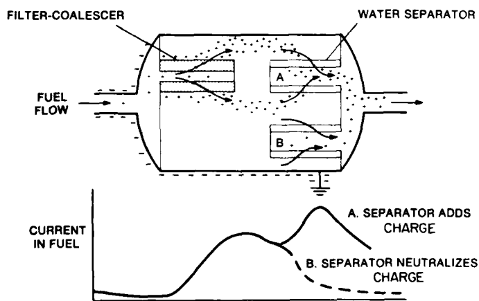
Fig. 3 — Charge separation in a filter/separator [2]
