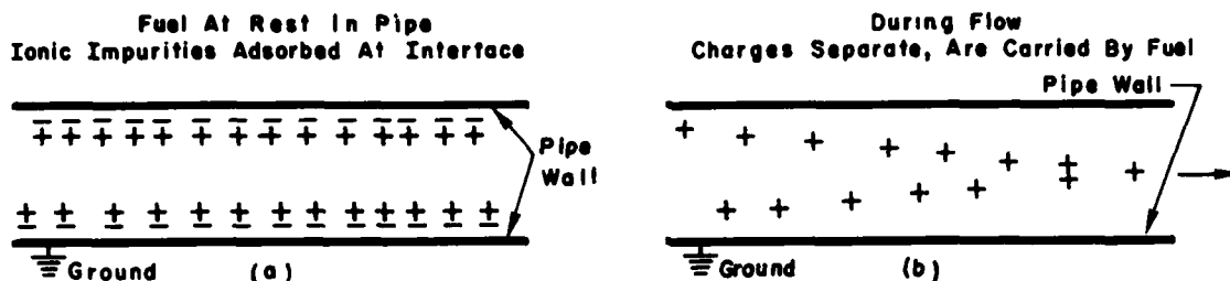
Fig. 1 - (a) Fuel at rest in a pipe showing adsorption of ionic impurities at pipe wall (b) Separation of charge as fuel flows through pipe.
