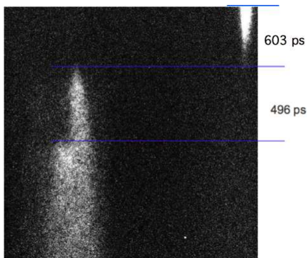
FIG. 3. Shock breakout image for a stepped target with E(3\omega) = 245 J, E pre-pulse = 29 J, and delay between auxiliary and main beam 500 ps (shot without phase plate on main beam).
