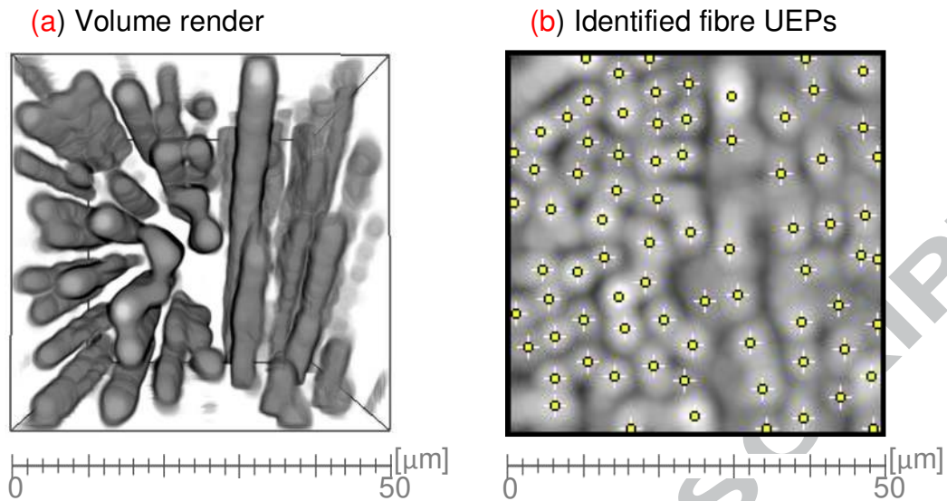
Fig. 7: Identification of the fibre centroids after image filtering in a RoI at the 0^\circ / -45^\circ ply boundary (bounding box corner= 255,1400,0 & 152 voxels): (a) volume render after image filtering and (b) identified UEPs in top image slice
