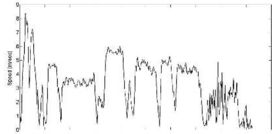
Figure 5. Speed of flight mission one (part two)
