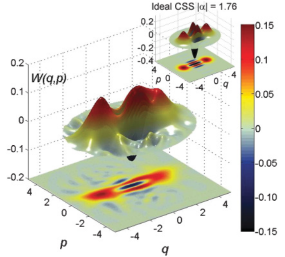
FIG. 4. (Color online) Maximum-likelihood estimate of an odd CSS after the subtraction of three photons from a squeezed vacuum. The reconstructed state has a fidelity of F = 0.592^{+0.036}_{-0.142} with a CSS of amplitude |\alpha| = 1.76^{+0.02}_{-0.19} . Inset, Wigner function of an ideal odd CSS with |\alpha| = 1.76 .
