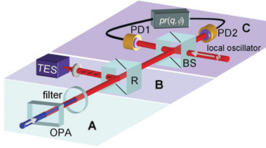
FIG. 1. (Color online) Scheme for optical CSS creation. An up-converted laser pulse enters an optical parametric amplifier (OPA) to create a squeezed vacuum state in section (A). After spectral filtering, this state is sent to a weakly reflecting beam splitter R in (B). Reflected photons that are detected herald a CSS emerging from R into (C). Its quadratures are measured by homodyne detection in (C).
