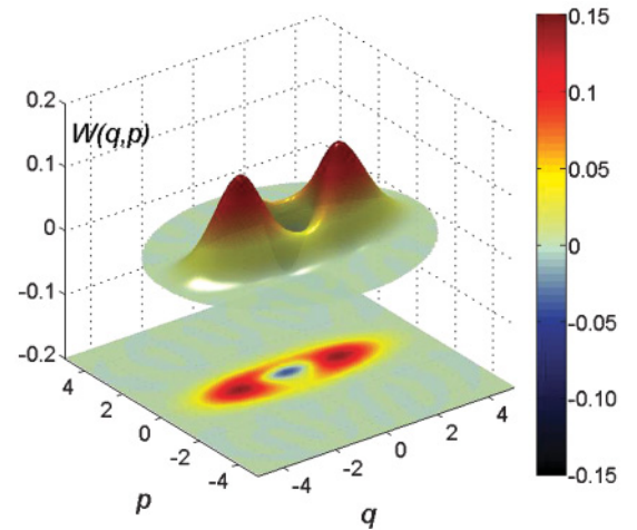
FIG. 2. (Color online) Maximum-likelihood estimate of an odd CSS generated by one-photon subtraction from a squeezed vacuum. The graph shows the unitless Wigner function value W(q, p) as a function of the unitless quadratures of the electromagnetic field.
