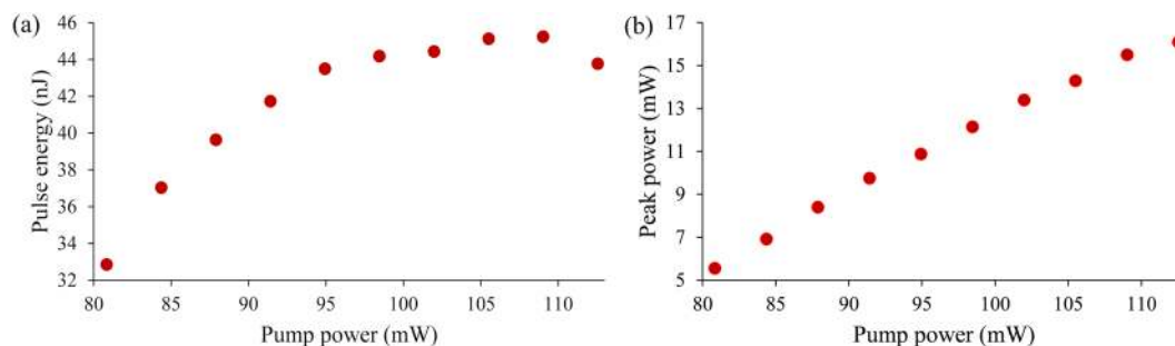
Figure 6. Output trend of TDFL (a) pulse energy and (b) peak power against pump power.
