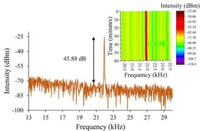
Figure 10. RF spectrum stability of THDFL at 123 mW over 60 minutes.
