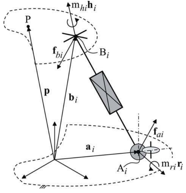
Figure 6. i^{\text{th}} limb of type nSPU: free-body diagram.
