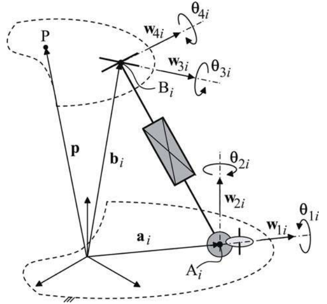
Figure 5. i^{\text{th}} limb of type nSPU: notations.
