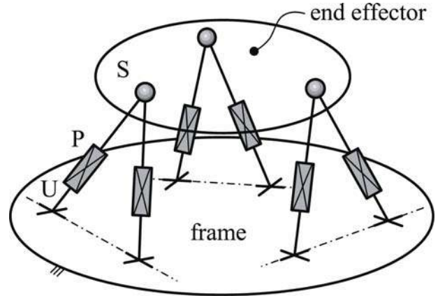
Figure 2. 6-3 FPM
