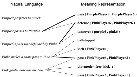
Figure 2: Sample trace from Robocup English data.
