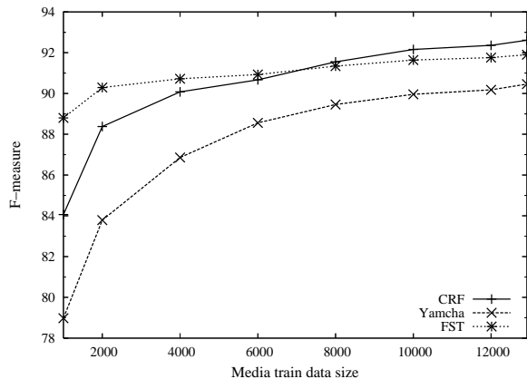
Figure 3: F -measure on MEDIA data learning curves
