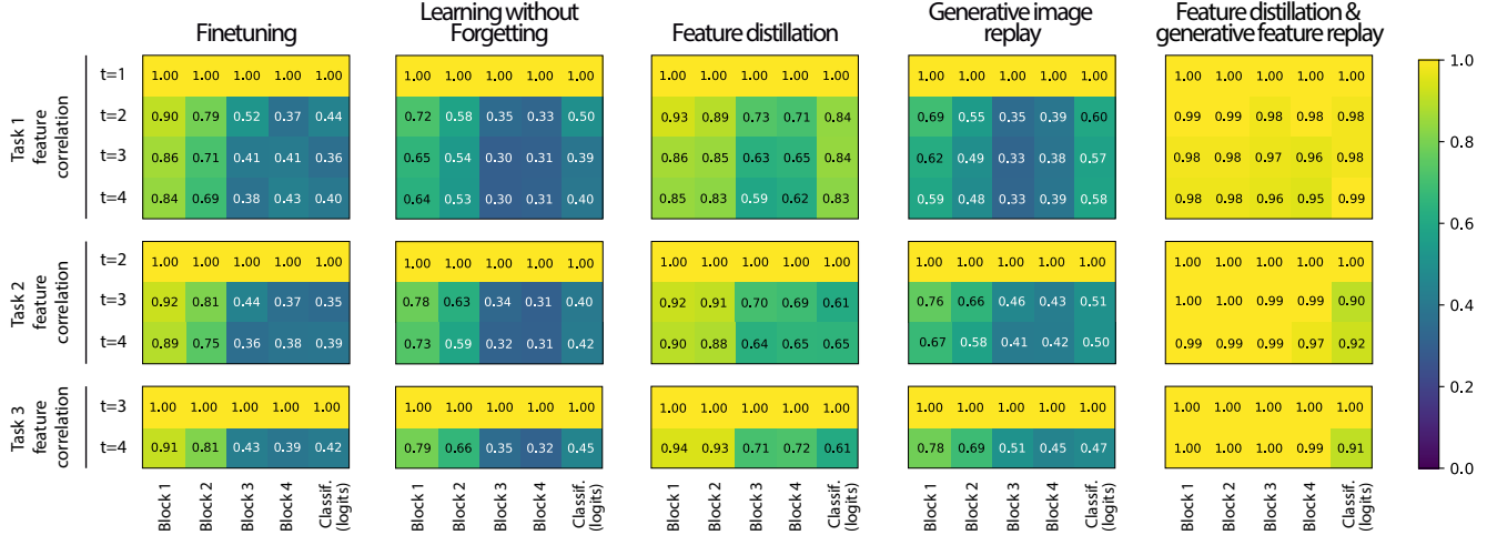
Figure 2. Canonical Correlation Analysis (CCA) similarity of different continual learning methods performed on equally distributed 4-task scenario on CIFAR-100. The vertical axis shows the evolution over time of the correlation for given task activations. The horizontal axis shows correlation at different layers of the network.
