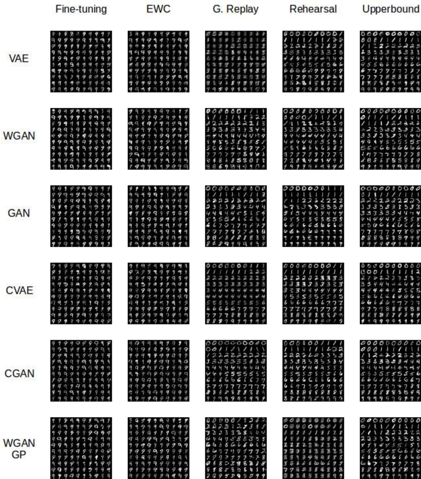
Fig. 14: MNIST samples for each generative model and each Continual Learning strategy, at the end of training on 10 sequential tasks. The goal is to produce samples from all categories.
