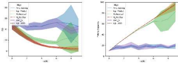
Fig. 2: Comparison, averaged over 8 seeds, between FID results(left, lower is better) and Fitting Capacity results (right, higher is better) with GAN trained on MNIST.
