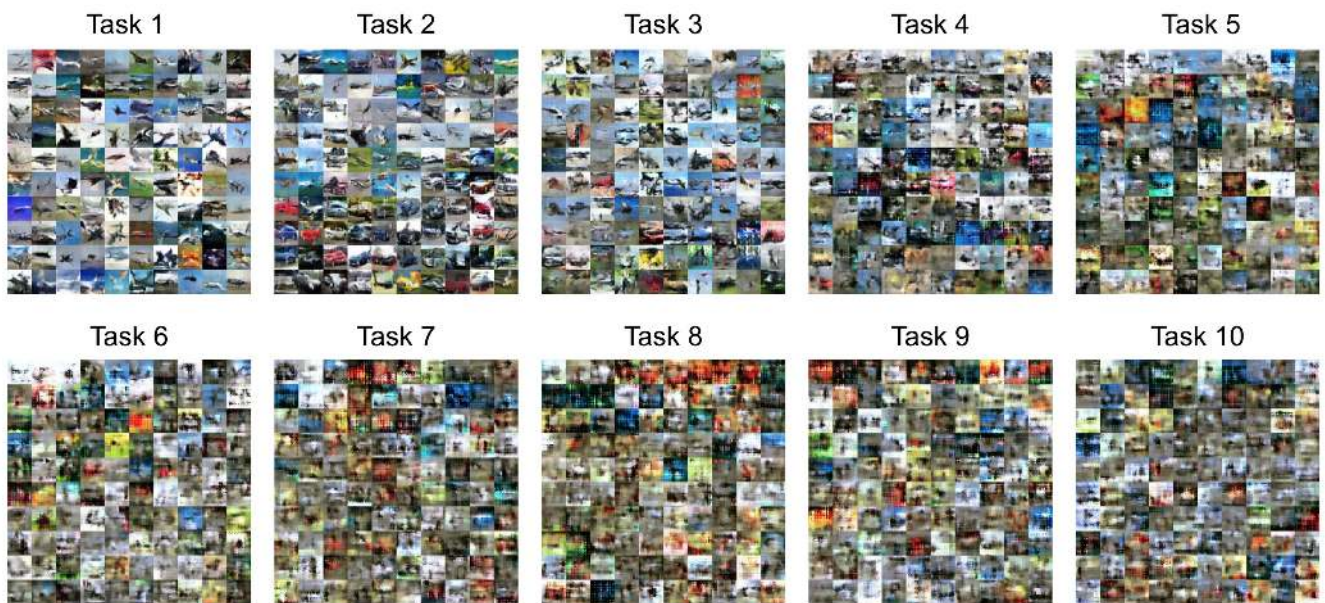
Fig. 17: WGAN-GP samples on 10 sequential tasks on CIFAR10, with Generative Replay. Classes, from 0 to 9, are planes, cars, birds, cats, deers, dogs, frogs, horses, ships and trucks. We observe that generation errors snowballs as tasks are encountered, so that the images sampled after the last task are completely blurry.
