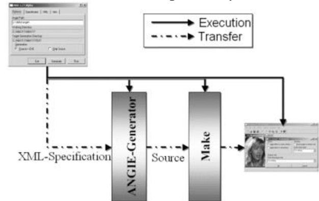
Figure 3. The generation process in ABA
