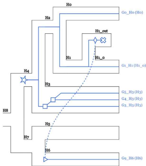
FIG. 4. Reconciled GFT and species tree. Users can easily visualize reconciliations inferred with GeneRax using the online tool RecPhyloXML-visu (Duchemin et al. 2018). This example illustrates one HGT and one duplication events.
