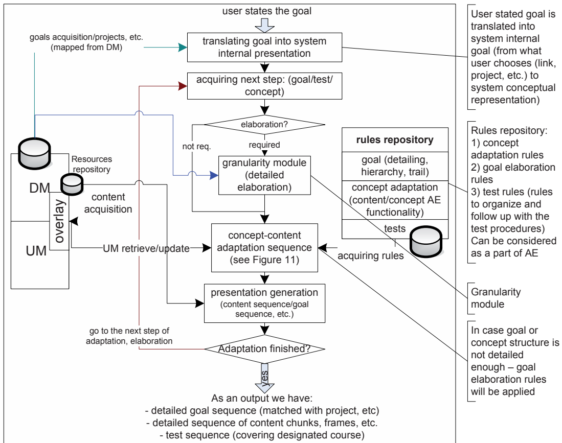
Figure 15: Use-Case: Adaptive Course flowchart
