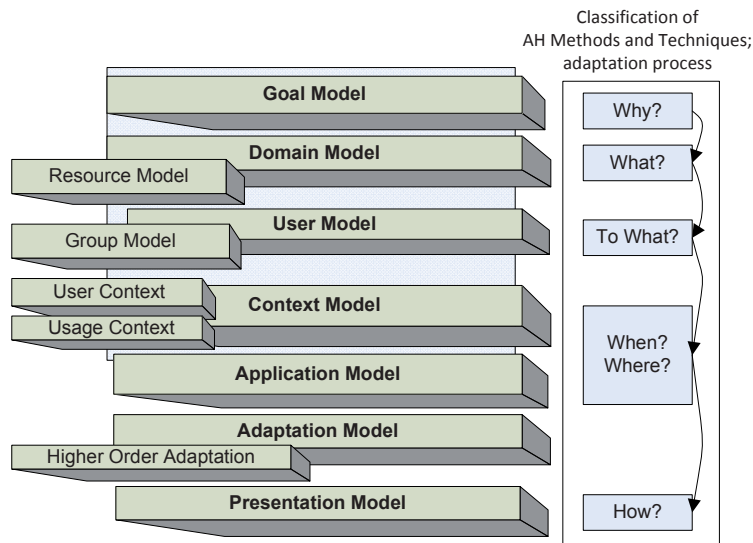
Figure 13: Conceptual scheme of a Generic Adaptation Framework (GAF)
