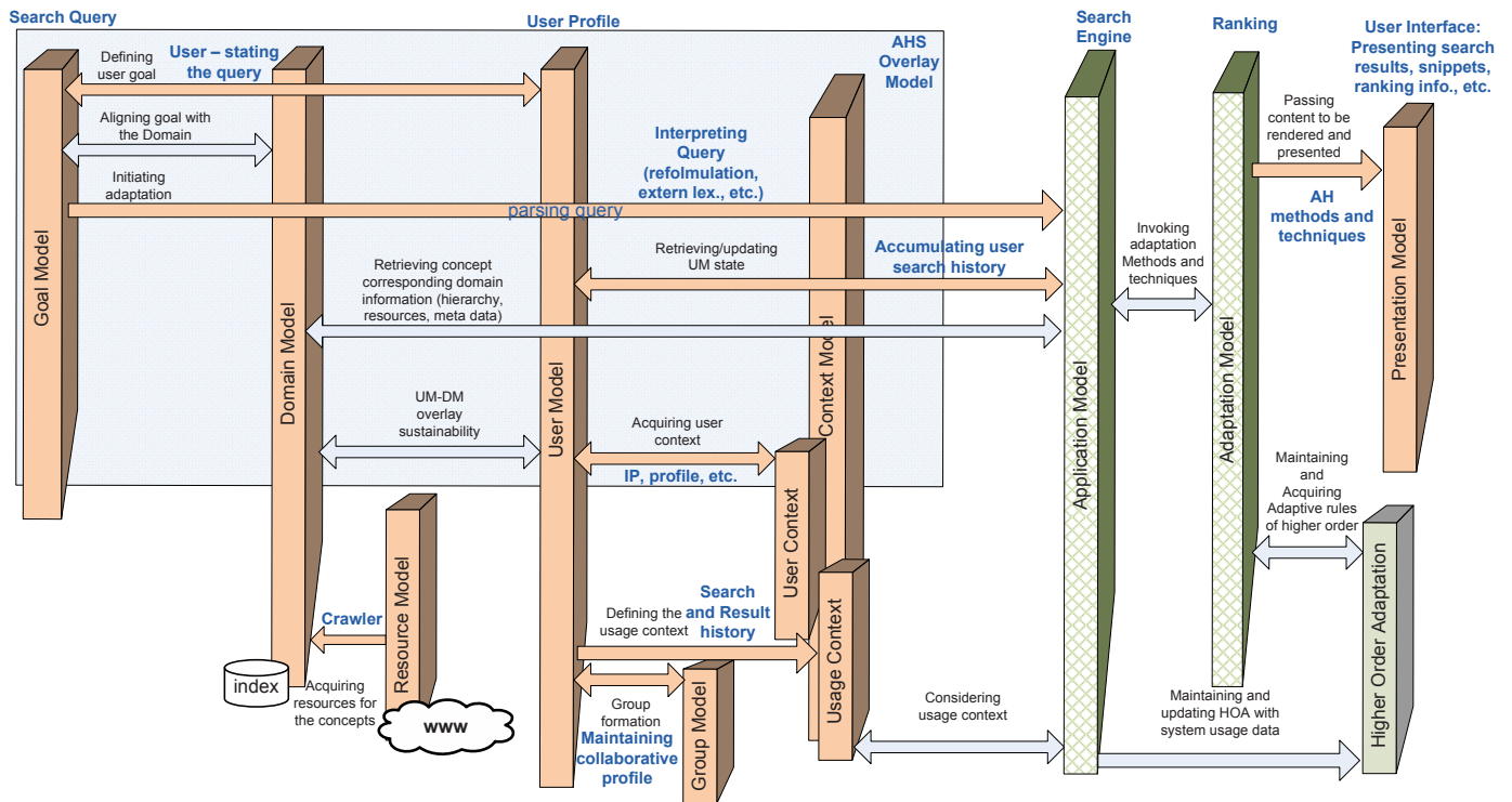
Figure 17: Search Compliance With Generic Adaptation Process
