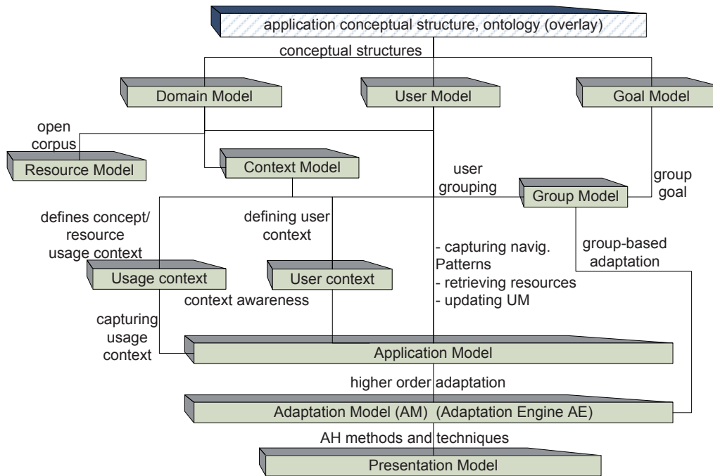
Figure 20: GAF layers hierarchy
