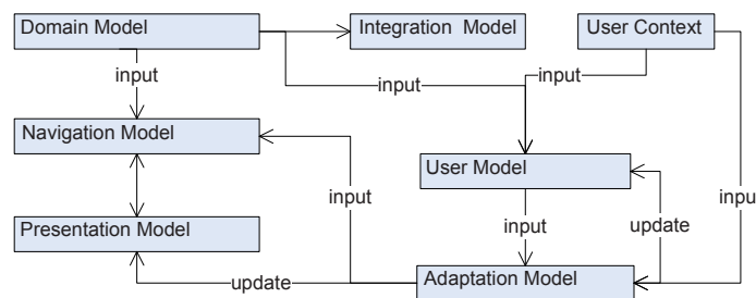
Figure 8: General meta-model for AHS
