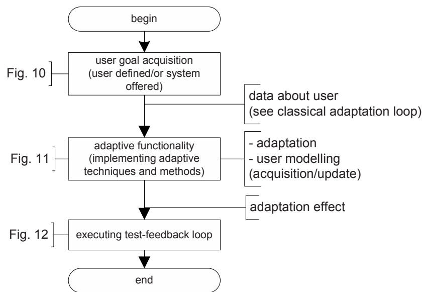
Figure 9: Generic Adaptation Flowchart (to be considered as the aggregation of Figures 10 - 12)
