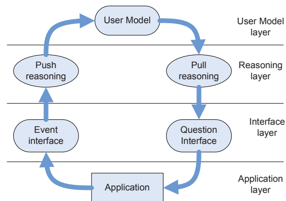
Figure 6: Overview of the Generic Adaptivity model
