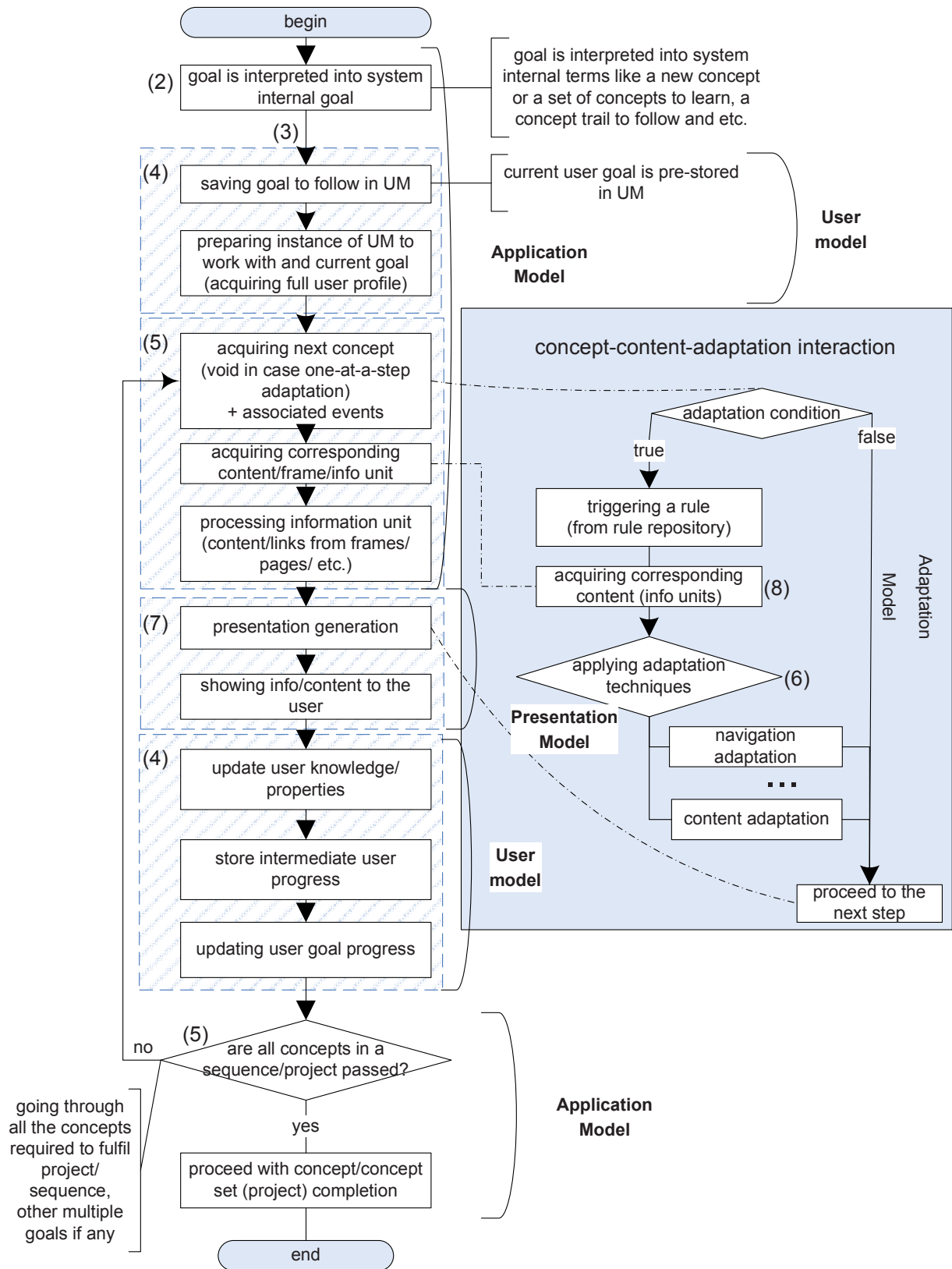
Figure 11: Adaptation functionality flowchart
