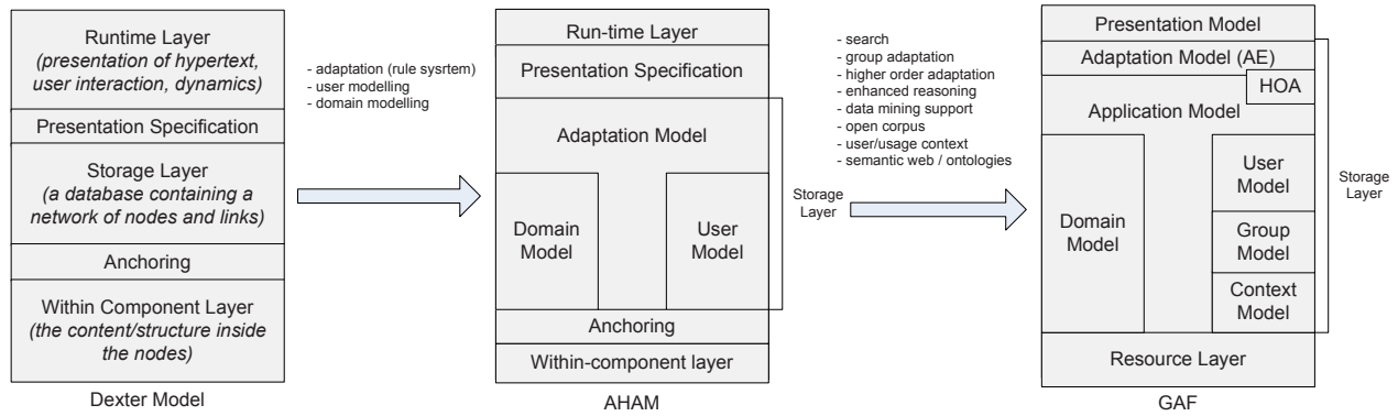
Figure 19: From Dexter, through AHAM, to GAF
