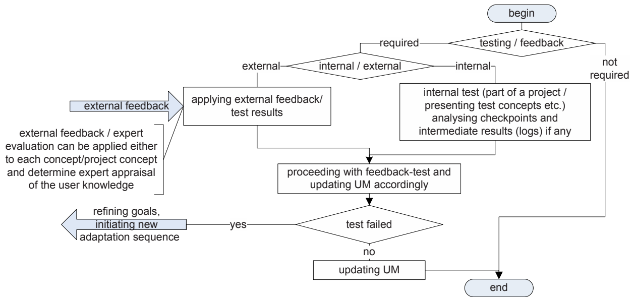
Figure 12: Test-feedback functionality flowchart
