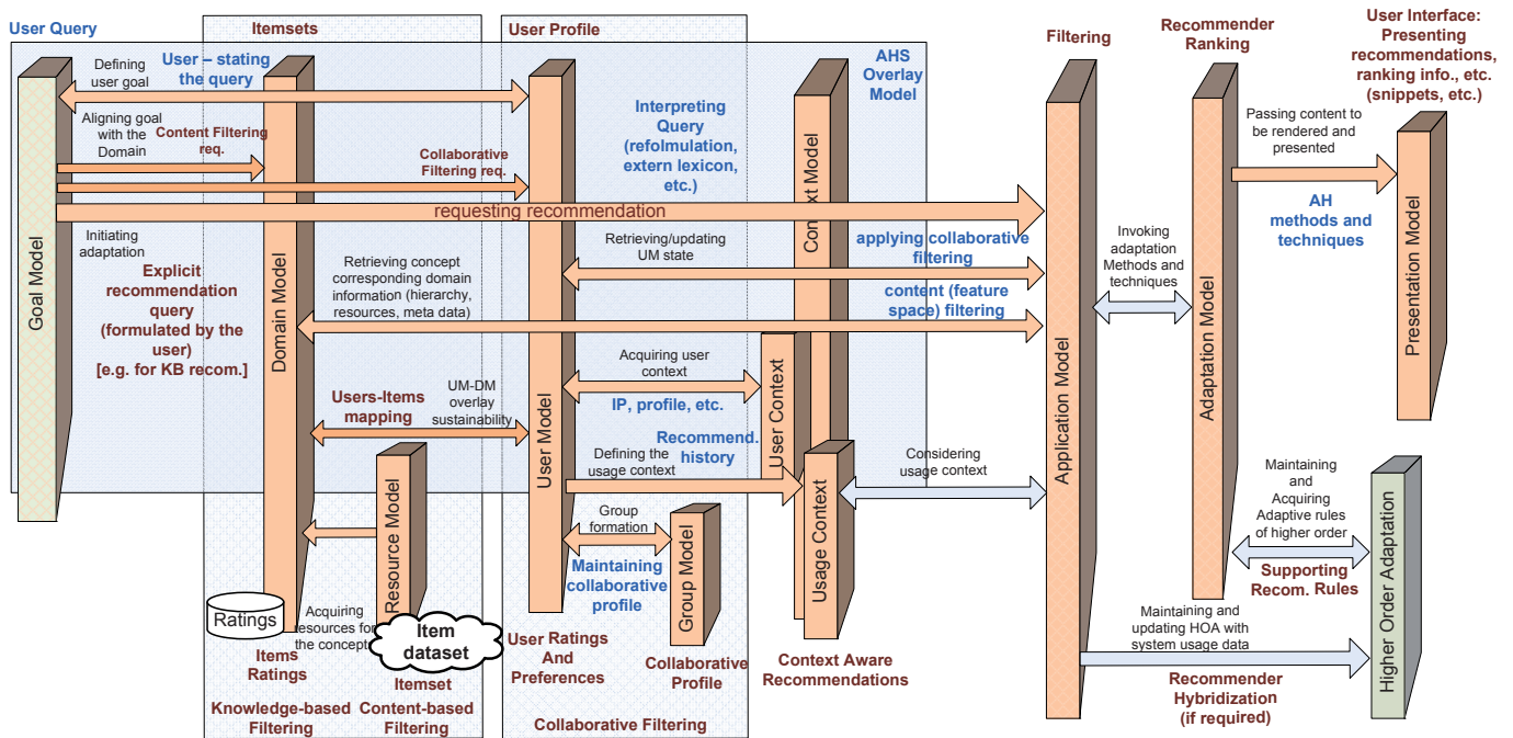
Figure 18: Recommender System Compliance With Generic Adaptation Process
