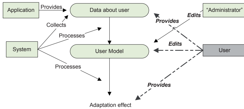
Figure 3: Collaborative user model editing (User and Administrator involved)
