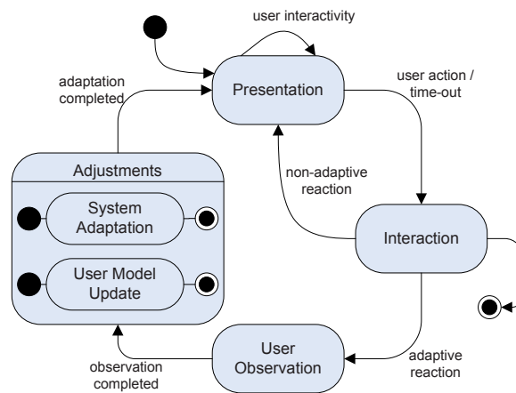
Figure 7: Lifecycle Model of Adaptation (Munich Model)
