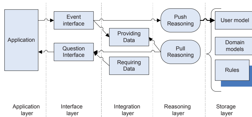
Figure 5: Overview of the General Ontological Model for Adaptive Web Environments (GOMAWE)
