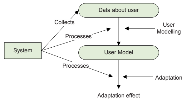
Figure 1: Classic loop user modelling - adaptation
