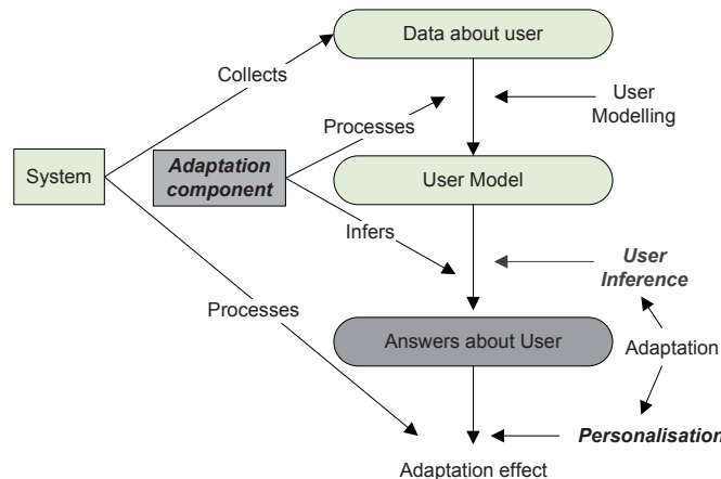
Figure 2: User model inference - adaptation loop
