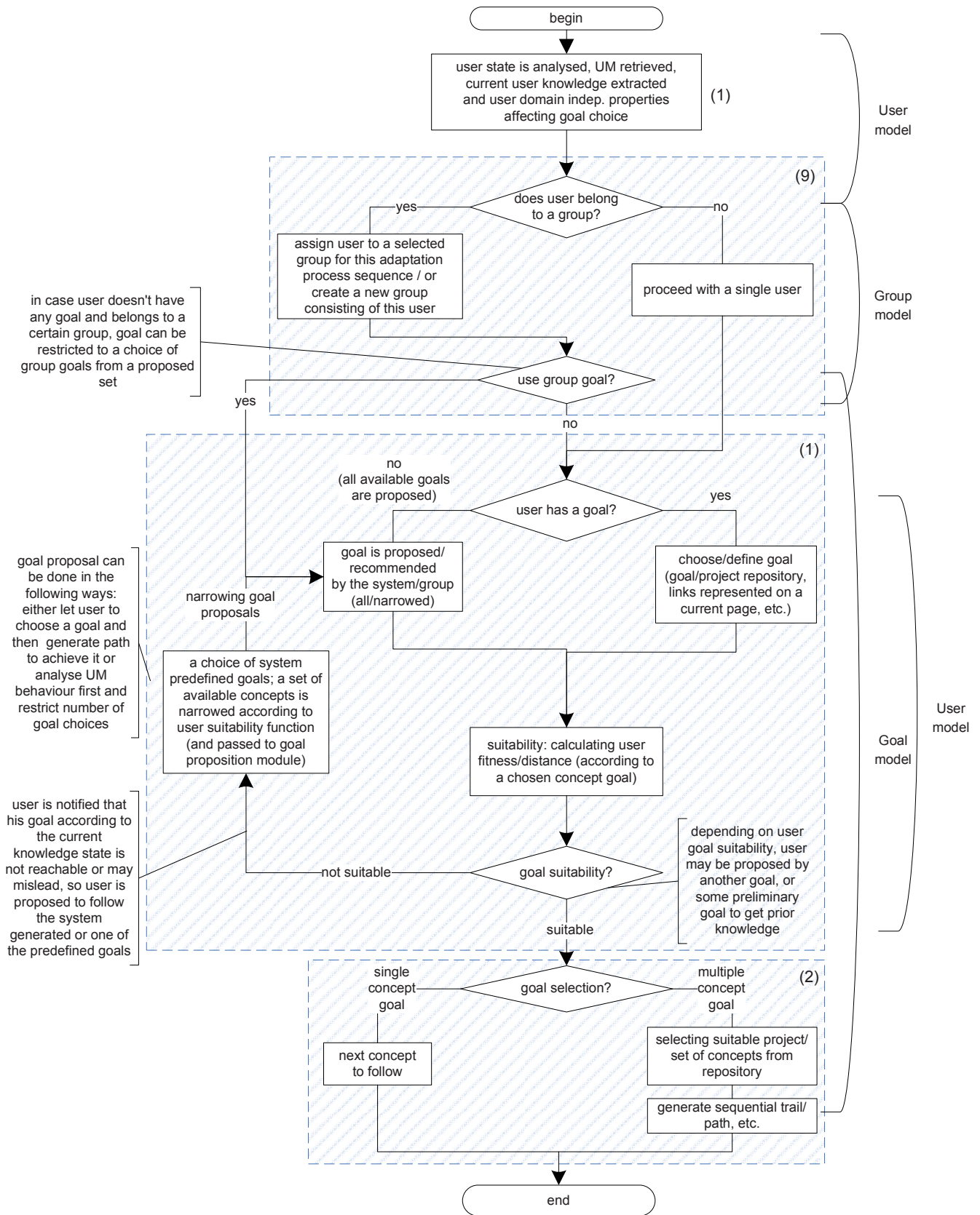
Figure 10: Goal acquisition and adaptation flowchart
