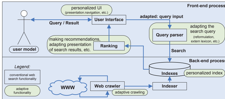
Figure 16: Web Search Schema
