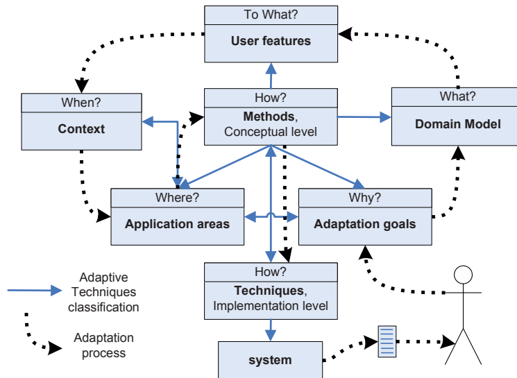
Figure 4: Classification of AH methods and techniques; adaptation process highlights (Knutov et al. 2009)
