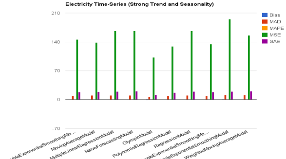
(b) Model performance on TimeSeries with seasonality.
