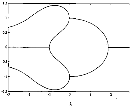
Figure 3. Imaginary parts of the eigenvalues in example (b) against the bifurcation parameter \lambda . The sequence splitting at 0 \rightarrow splitting at \pm 1 can be observed as \lambda is varied. The last eigenvalue bifurcation is related to splitting off the real axis , but this does not correspond to a dynamic bifurcation.
