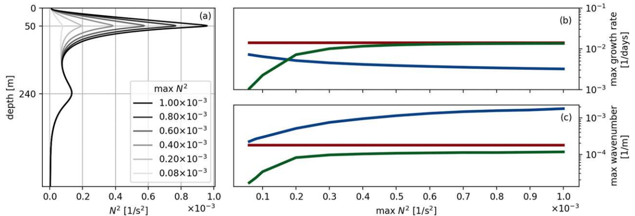
FIG. 6. (a) Variability in the peak value of stratification affects the (b) growth rate and (c) wavenumber of the fastest growing perturbation. Ekman layer depth is fixed at 5 m. Colors as in Fig. 4.
