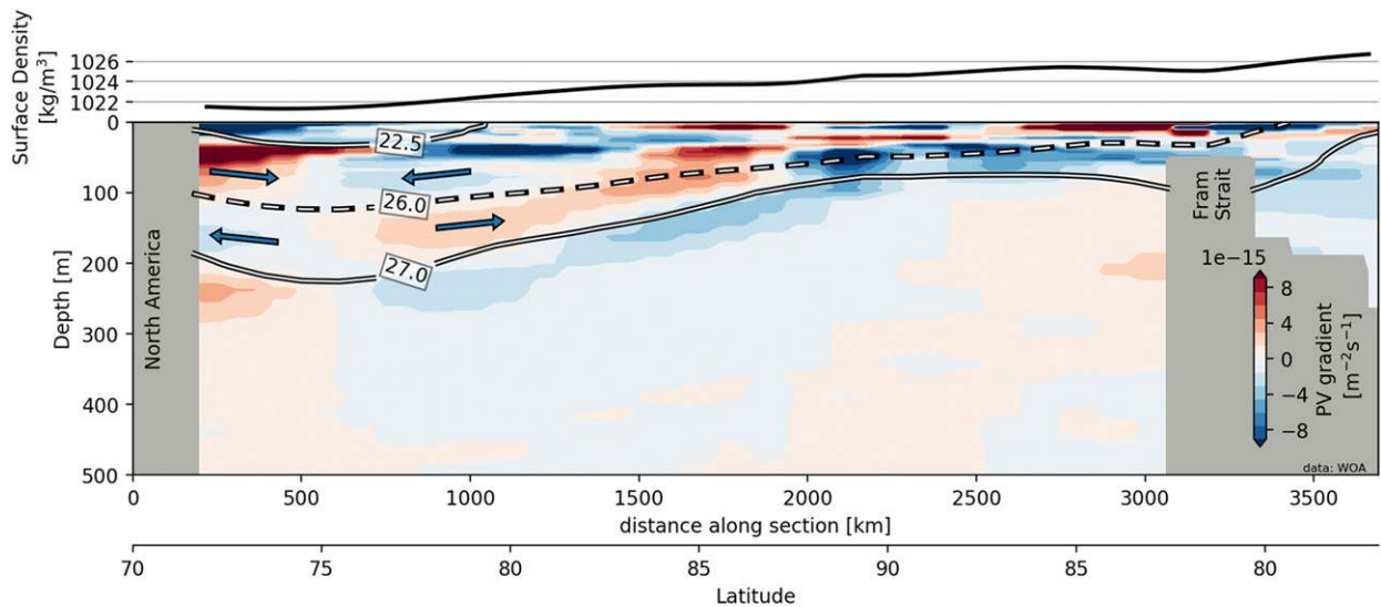
FIG. 9. (top) Surface density and (bottom) Ertel PV gradient \nabla[-(f/\rho)(\partial\rho/\partial z)] along the same section as Fig. 2. The PV gradient reversal with depth, marked for example by blue arrows in the Canadian basin halocline, supports the growth of halocline eddies independently of the presence of sea ice. Contours mark the 22.5, 27 (solid lines), and 26 \text{kg m}^{-3} (dashed) isopycnals. Data from the 2005–17 World Ocean Atlas climatology.
