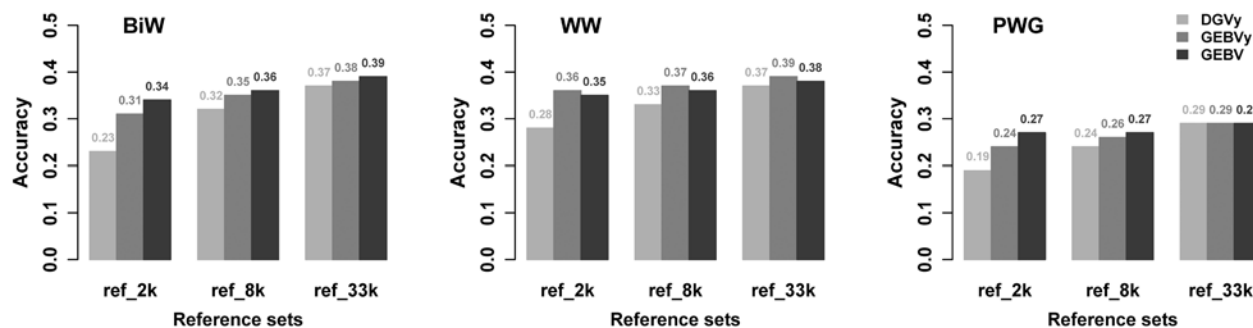
Figure 1. Predictive ability of indirect predictions on 18,721 young genotyped animals when using reference populations ref_2k (contains top bulls and top cows that had an EBV accuracy for BiW \geq 0.85 ), ref_8k (contains all parents that were genotyped) ref_33k (contains all genotyped animals born up to 2012) animals to run single-step genomic BLUP (ssGBLUP) and derive SNP effects. BiW = birth weight; WW = weaning weight; PWG = postweaning gain; DGV y = direct genomic value for young genotyped animals; GEBV y = is genomic estimated breeding value obtained via indirect predictions for young animals and DGV y . GEBV (genomic estimated breeding value, obtained directly from ssGBLUP when genotypes on reference and validation animals were considered together in evaluations are genomic predictions obtained directly from ssGBLUP when genotypes on reference and validation animals were considered together in evaluations. Predictive ability was calculated as correlation between corrected phenotypes and genomic EBV.
