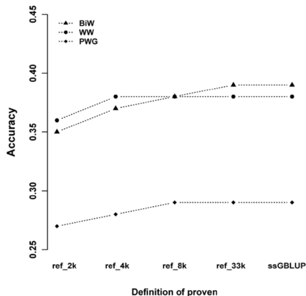
Figure 2. Predictive ability of genomic estimated breeding value for 18,721 young genotyped animals when using the algorithm for proven and young animals to invert the G matrix (genomic-based relationship matrix) with different definitions of proven animals: ref_2k (contains top bulls and top cows that had an EBV accuracy for BiW \geq 0.85 ), ref_4k (contains genotyped parents of genotyped animals), ref_8k (contains all parents that were genotyped) ref_33k (contains all genotyped animals born up to 2012). Predictive ability was calculated as correlation between corrected phenotypes and genomic EBV. Predictions in single-step genomic BLUP (ssGBLUP) are obtained through direct inversion of G . BiW = birth weight; WW = weaning weight; PWG = postweaning gain.
