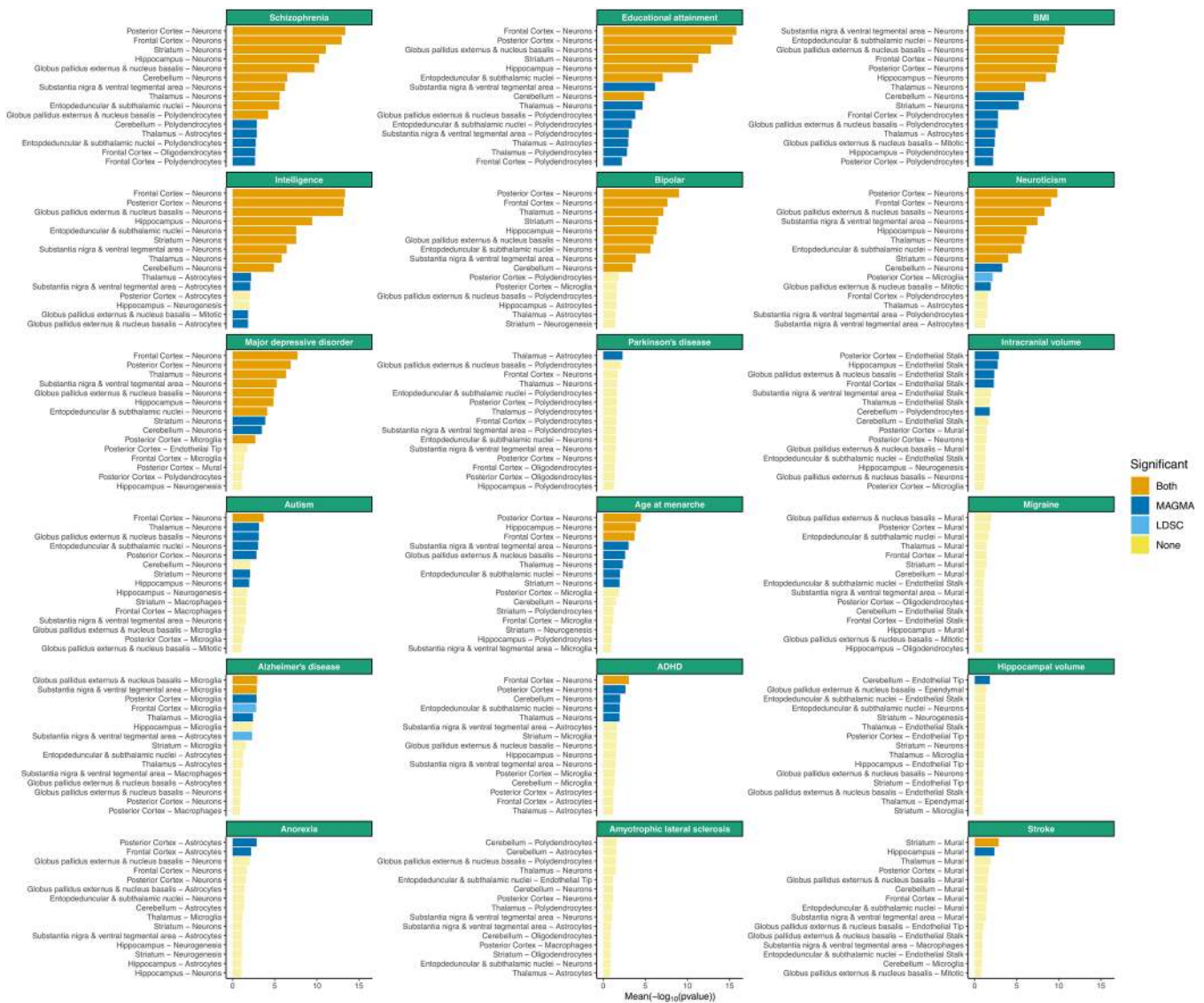
Extended Data Fig. 6 | Replication of cell type—trait associations in 88 cell types from 9 different brain regions. The mean strength of association ( -\log_{10}P ) of MAGMA and LDSC is shown for the 15 top cell types for each trait. The bar color indicates whether the cell type is significantly associated with both methods, one method or none (significance threshold: 5% false discovery rate).
