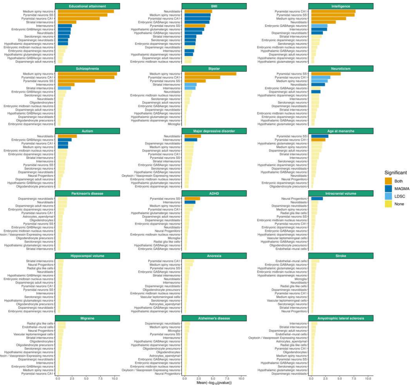
Extended Data Fig. 9 | Top associated cell types with brain related traits among 24 cell types from 5 different brain regions. The mean strength of association (-log 10 P) of MAGMA and LDSC is shown for the 15 top cell types for each trait. The bar color indicates whether the cell type is significantly associated with both methods, one method or none (significance threshold: 5% false discovery rate).
