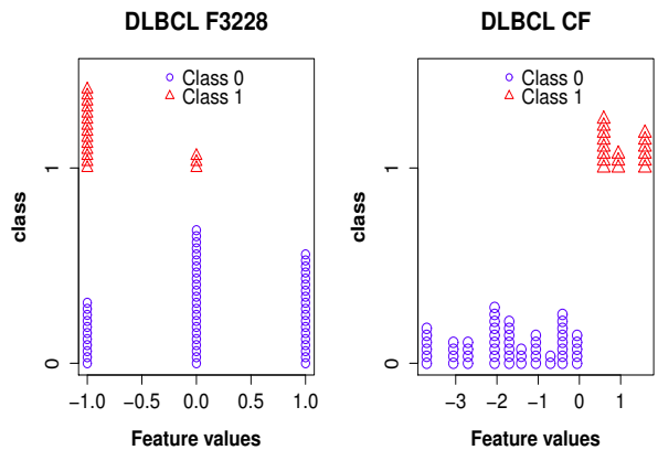
Fig. 7 DLBCL Feature F3228 and the Constructed Feature.
