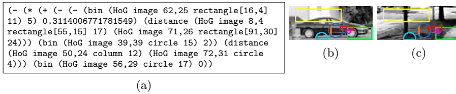
Fig. 5. Example program 3: 96% training and 97% test performance on UIUC dataset (a) Lisp expression, (b) Car (+ve) image, and (c) Background (-ve) image.
