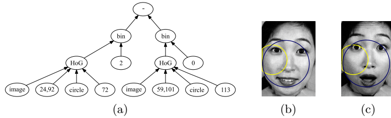
Fig. 4. Example program 2: 95% training and 100% test performance on Jaffe dataset (a) GP tree, (b) Happy (+ve) expression, and (c) Surprised (-ve) expression.
