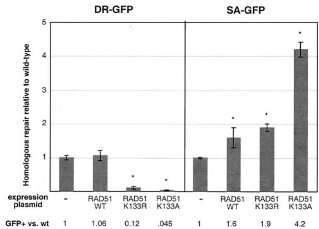
FIG. 2. RAD51-K133R and RAD51-K133A expression reduces HDR but increases SSA. Wild-type (wt) ES cells with either the DR-GFP or SA-GFP reporter were cotransfected with the I-SceI and RAD51 expression vectors, as indicated. The efficiency of homologous repair is indicated relative to transfection with the I-SceI expression vector alone, which is set to 1. The asterisks indicate a statistically significant difference from transfection with the I-SceI expression vector alone, with P \leq 0.0001 , except for SA-GFP repair with RAD51-WT, with P = 0.02 . The error bars indicate standard deviations.
