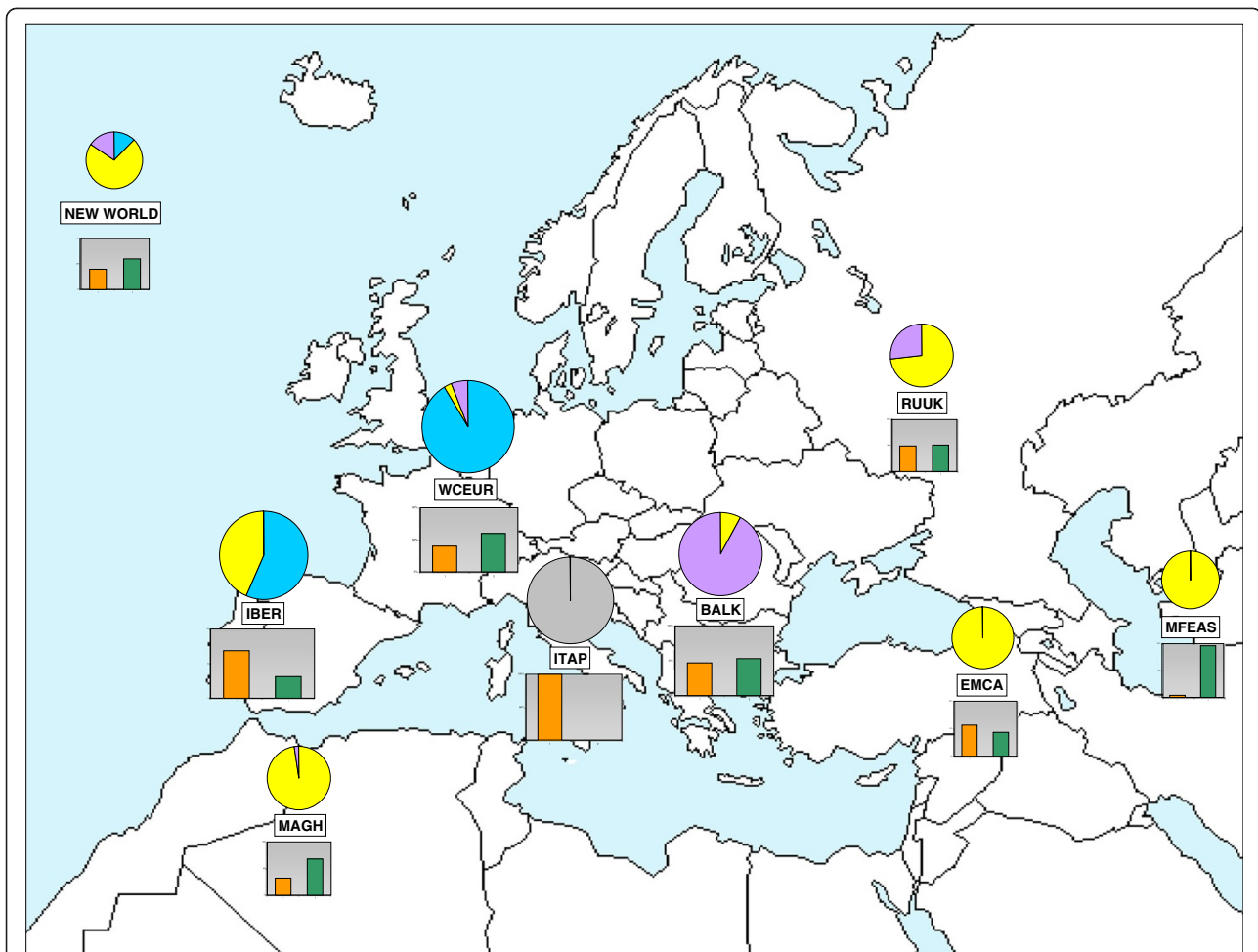
Figure 3 Genetic composition of the geographic groups. Genetic composition of the geographic groups for the K_s = 3 of STRUCTURE. For the detailed country list, see Table 1. The histograms represent the percentage of non-admixed (green) versus admixed (orange) genotypes. For the non-admixed cultivars, the pies represent the proportion of each cluster in each region: Table / East (yellow); Wine / Balkans and East-Europe (violet); Wine / West and Central Europe (blue). As 100% of the Italian genotypes are admixed, the ITAP pie is empty (grey).
