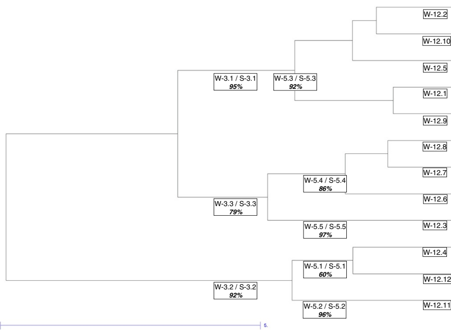
Figure 5 Dendrogram based on Ward's clustering. Dendrogram based on Ward's clustering. For levels three and five of clustering, the comparison among the Ward and STRUCTURE groups is summarized with the double code labels (W-x.x / S-x.x), and the percentage of shared individuals between them.
