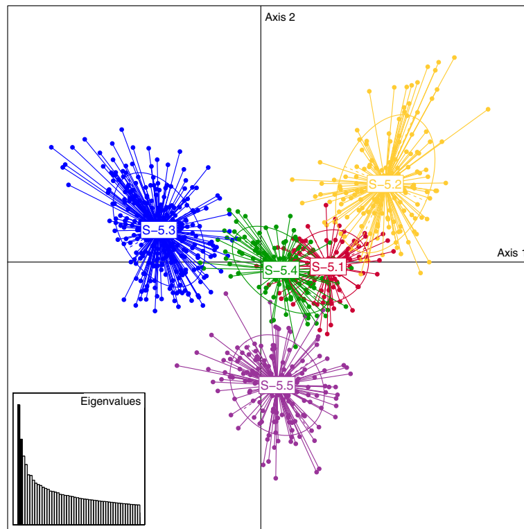
Figure 4 Principal component analysis on SSR data. Principal component analysis on SSR data of genotypes belonging to Ks = 5. Colors of the groups correspond to the colors in Figure 2. Axes 1 and 2 explain 30.3% and 21.4% of the total variance respectively (black vertical bars in the eigenvalues histogram).
