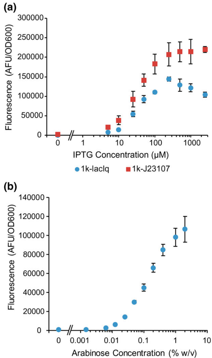
Fig. 2. Induction curves for BglBrick promoter systems in P. putida . a Induction curves for 1k promoter system with P_{lacIq} and J23107 promoters expressing lacI . b Induction curve for 8k system. Error bars represent one standard deviation. Fluorescence values are adjusted so that the empty vector control has a value of 0
