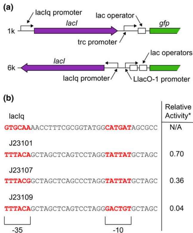
Fig. 1. IPTG-inducible promoter systems from the BglBrick vector database. a Genetic structure of the 1k and 6k promoter systems, highlighting the promoters used and the direction of lacI expression. b Sequences of P lacIq and the three Anderson promoters used to modify the 1k and 6k promoter systems. The — 10 and — 35 motifs are highlighted in red. (Asterisk) Relative activity is the promoter strength in E. coli with respect to the reference promoter in the Anderson promoter library, J23100 (color figure online)
