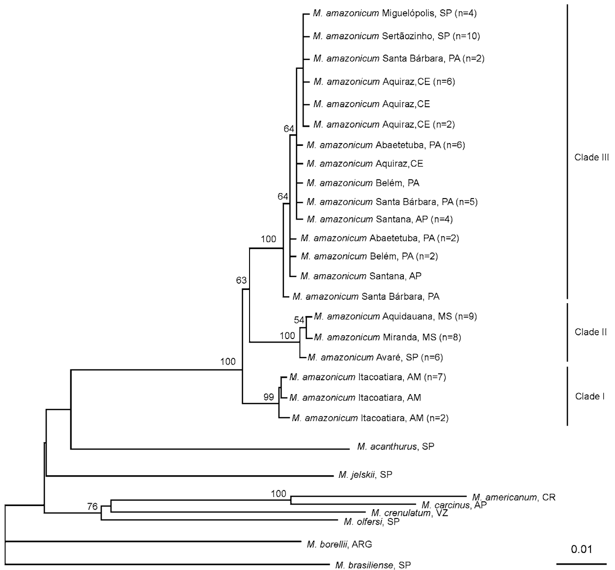
Fig. 5. Dendrogram for Macrobrachium amazonicum populations from Brazil based on Neighbor-Joining analysis of COI gene sequences. Numbers above are significance values for 1000 bootstraps; values \leq 50\% are not shown. ARG: Argentina. CR: Costa Rica. VZ: Venezuela. Brazilian states: AM: Amazonas; AP: Amapá; CE: Ceará; MS: Mato Grosso do Sul; PA: Pará; SP: São Paulo. Clades: I - inland population from Amazonian Hydrographic Region (HR); II - inland populations from Paraná/Paraguay HR; III - coastal populations from northern and north-eastern Brazil.
