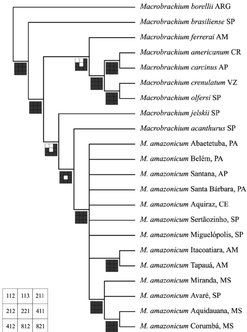
Fig. 2. Phylogenetic tree for populations of Macrobrachium amazonicum from Brazil based on direct optimization analysis of 16S rRNA data sets. The box on the left/down side indicates the parameter sets used in the sensitivity analysis. Filled boxes correspond to the parameters under which the clade was stable. ARG: Argentina. CR: Costa Rica. VZ: Venezuela. Brazilian states: AM: Amazonas; AP: Amapá; CE: Ceará; MS: Mato Grosso do Sul; PA: Pará; SP: São Paulo.
