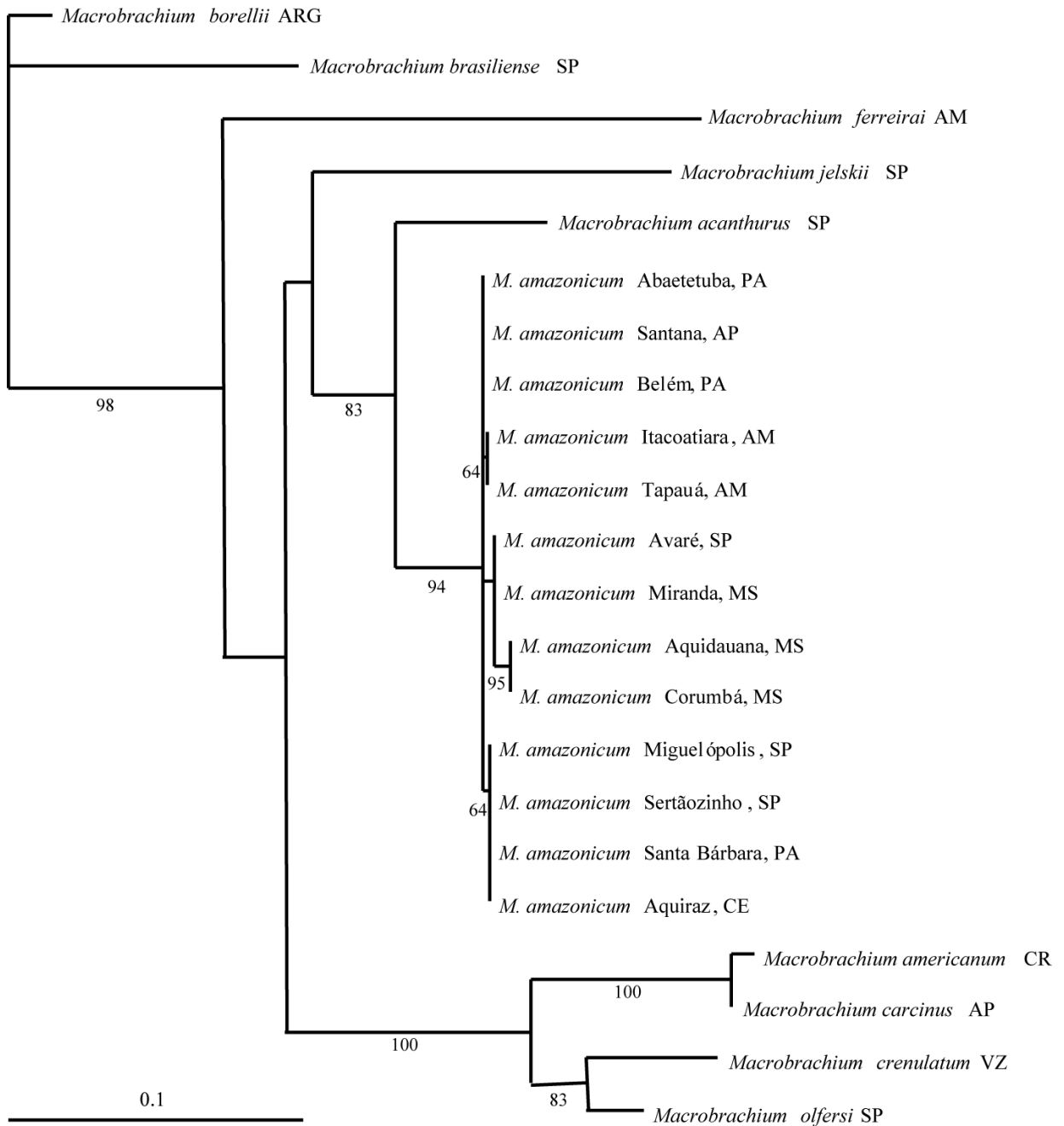
Fig. 4. Dendrogram for Macrobrachium amazonicum populations from Brazil based on Neighbor-Joining analysis of 16S rRNA gene sequences. Numbers above are significance values for 1000 bootstraps; values \leq 50\% are not shown. ARG: Argentina. CR: Costa Rica. VZ: Venezuela. Brazilian states: AM: Amazonas; AP: Amapá; CE: Ceará; MS: Mato Grosso do Sul; PA: Pará; SP: São Paulo.
