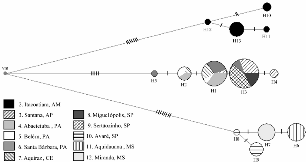
Fig. 6. Haplotype network based on Median-Joining analysis indicating the distribution of each haplotype (H) found in Macrobrachium amazonicum . The haplotype identification is below each circle. Circle size for each haplotype is proportional to the overall frequency in our sample. Each small trace represents a mutational step. vm: median vector. The numbers before the sample site name in the legend boxes correspond to the ones used in Fig. 1. Brazilian states: AM: Amazonas; AP: Amapá; CE: Ceará; MS: Mato Grosso do Sul; PA: Pará; SP: São Paulo. Groups: I - inland population from Amazonian Hydrographic Region (HR); II - inland populations from Paraná/Paraguay HR; III - coastal populations from northern and north-eastern Brazil.
