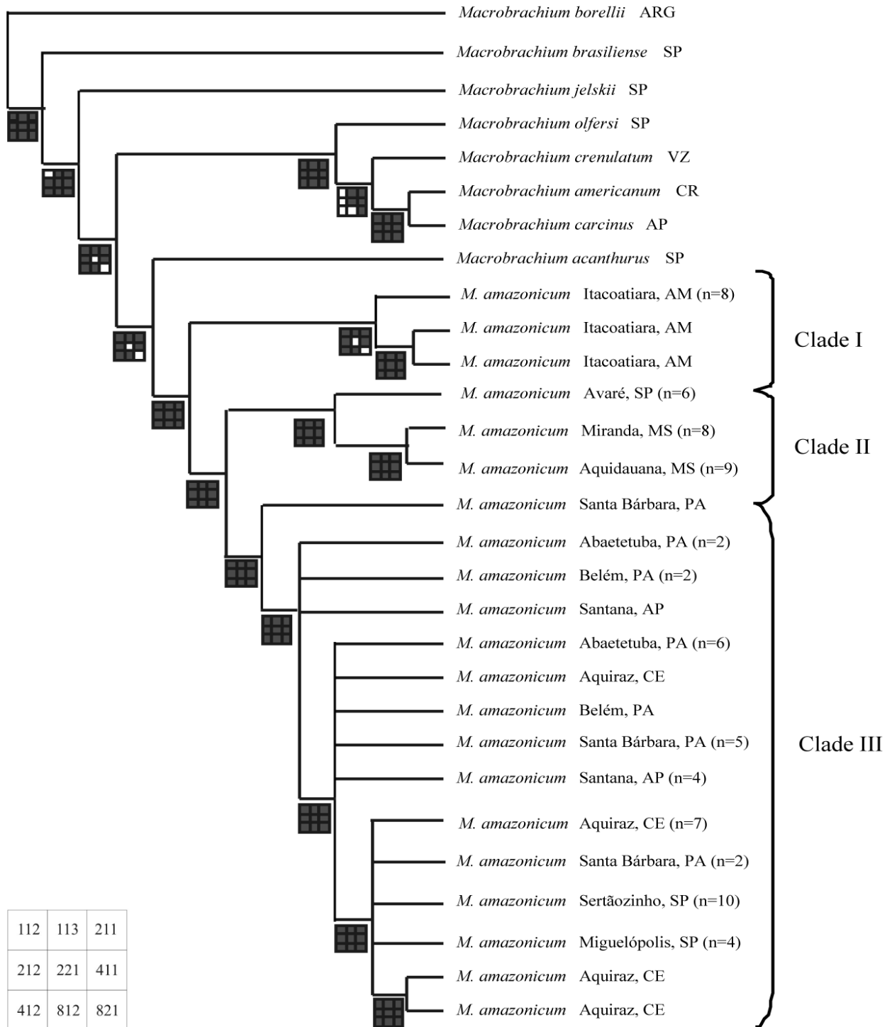
Fig. 3. Phylogenetic tree for populations of Macrobrachium amazonicum from Brazil based on direct optimization analysis of COI data sets. The box on the left/down side indicates the parameter sets used in the sensitivity analysis. Filled boxes correspond to the parameters under which the clade was stable. ARG: Argentina. CR: Costa Rica. VZ: Venezuela. Brazilian states: AM: Amazonas; AP: Amapá; CE: Ceará; MS: Mato Grosso do Sul; PA: Pará; SP: São Paulo. Clades: I - inland population from Amazonian Hydrographic Region (HR); II - inland populations from Paraná/Paraguay HR; III - coastal populations from northern and north-eastern Brazil.
