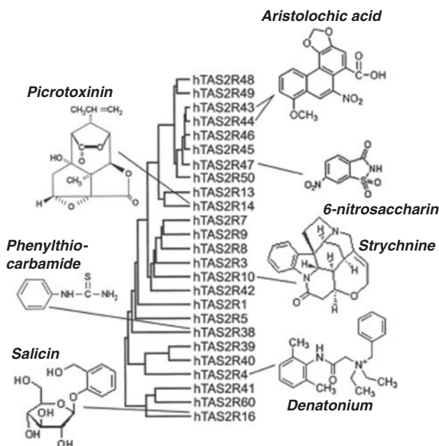
Fig. 2. Phylogenetic tree of members of the TAS2R gene family and some of the ligands which bind their receptors (taken from Behrens and Meyerhof (99) ).
