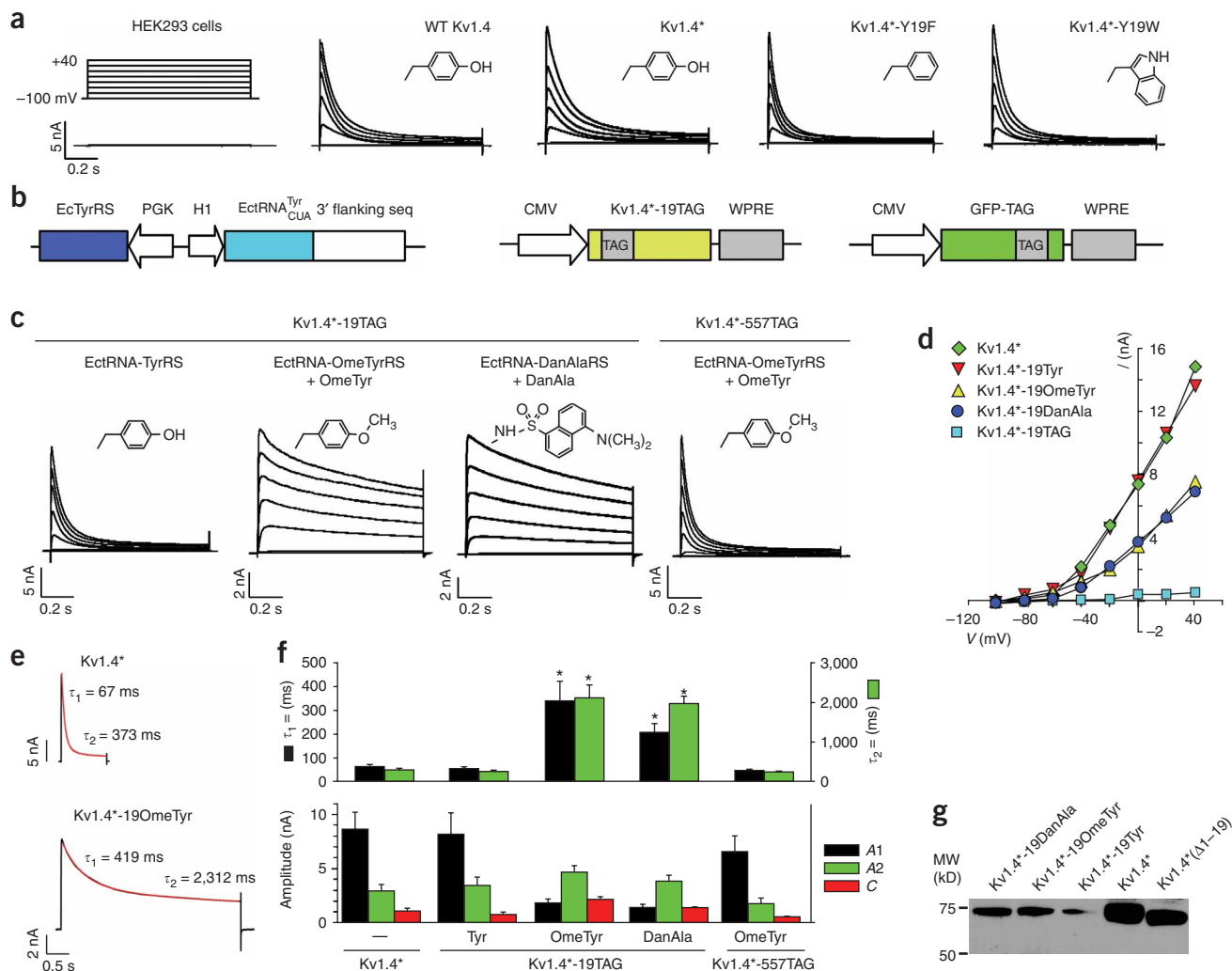
Figure 5 Probing N-type inactivation using unnatural amino acid mutagenesis with Kv1.4 channels expressed in mammalian cells. (a) Comparison of macroscopic currents recorded from HEK293 cells expressing wild-type Kv1.4, Kv1.4* (Kv1.4-M109L), Kv1.4*-Y19F or Kv1.4*-Y19W channels. Untransfected HEK293 cells displayed a small, background current ( 0.50 \pm 0.03 nA, n = 5 ). Inserts in each panel show the side-chain structures of amino acids at position 19. (b) Constructs for expressing Kv1.4 through amber suppression. The GFP-TAG reporter plasmid was used as an indicator for transfection. (c) Potassium currents recorded from HEK293 cells expressing Kv1.4*-TAG channels through amber suppression using the indicated orthogonal tRNA-synthetase pair. Only background currents were recorded for Kv1.4*-19TAG alone ( 0.40 \pm 0.05 nA, n = 5 ) or Kv1.4*-TAG with the EctRNA-OmeTyrRS pair in the absence of OmeTyr ( 0.42 \pm 0.07 nA, n = 4 ). The Kv1.4*-19OmeTyr and Kv1.4*-19DanAla mutants exhibited significantly slower inactivation than Kv1.4* and Kv1.4*-19Tyr. Inserts in each panel are the side chain structures. (d) Peak current plotted as a function of voltage for the indicated Kv1.4 channels. (e) Current (black trace) elicited by a 1-s (Kv1.4*) or 4-s (Kv1.4*-19OmeTyr) voltage step to +20 mV were fit with a sum of two exponentials (red line) relaxing to a small steady-state current with the indicated time constants. (f) Quantitative analysis of inactivation kinetics. Bar graphs show the average time constants ( \tau_1 , \tau_2 ) for the fast and slow inactivation components, current amplitudes ( A_1 , A_2 ) for the exponentials and steady-state current ( C ). Specific values are in Table 1. Asterisks indicate statistical difference from Kv1.4* ( P < 0.05 ). (g) Western blot analysis of Kv1.4*-19OmeTyr and Kv1.4*-19DanAla. The full-length Kv1.4*, Kv1.4*-19Tyr, and a truncated Kv1.4* with the first 19 amino acid residues deleted were run as controls.
