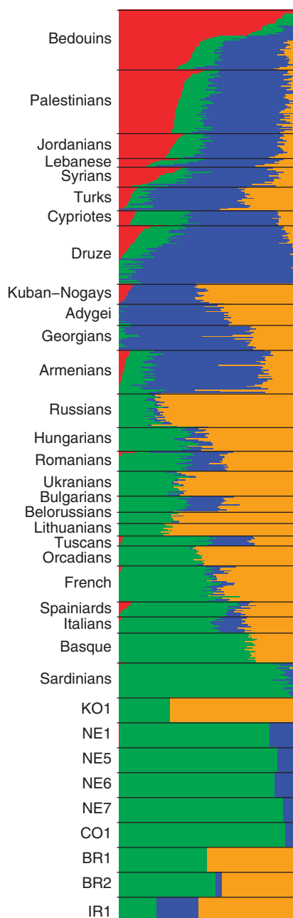
Figure 4 | Ancient Hungarians ADMIXTURE plot. ADMIXTURE analysis ( K=4 ) of the nine 1\times imputed samples along with 552 modern reference samples (HGDP+) using a LD ( r^2<0.2 ) filtered data set of 60,824 SNPs.
