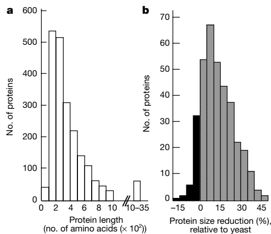
Figure 2 Sizes of E. cucuruli ( Ec ) proteins and comparison with S. cerevisiae ( Sc ) homologues. a , Distribution of the lengths of all the potential E. cucuruli protein chains. Only six have more than 2,000 amino acids (maximum 3,456 amino acids). b , Degrees of reduction in length of E. cucuruli proteins ( n = 350 ) relative to those of S. cerevisiae , expressed as a percentage: 100(\text{Sc protein length} - \text{Ec protein length})/(\text{Sc protein length}) . The positive classes representative of shorter E. cucuruli proteins are in grey. The dynein heavy chain, the largest protein chain with a clearly predicted function (3,151 amino acids), is \sim 23\% shorter than the yeast homologue (4,092 amino acids). Mean values associated with major functional categories are 7.3% for 'protein synthesis', 11.0% for 'protein destination', 11.4% for 'metabolism/energy', 14.4% for 'intracellular transport', 15.3% for 'transcription' and 20.1% for 'cell growth, cell division and DNA synthesis'.
