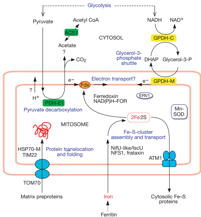
Figure 4 Conceptual scheme of a mitochondrion-derived organelle ('mitosome') in E. cucullii suggested by the detection of several homologues of mitochondrial proteins. Under this hypothesis, pyruvate decarboxylation may occur through a heterotetrameric form ( \alpha 2\beta 2 ) of the pyruvate dehydrogenase E1 component (PDH-E1) and transfer of reducing power towards the organelle transits through a glycerol-3-phosphate shuttle involving both cytosolic (GPDH-C) and mitochondrial (GPDH-M) glycerol-3-phosphate dehydrogenases. By analogy with hydrogenosomal pyruvate:ferredoxin oxidoreductase, a system based on ferredoxin (Fdx) and NAD(P)H ferredoxin:oxidoreductase (FOR) is assumed to be used for acetate production. A cytosolic acetyl coenzyme A (CoA) synthetase (ACS1) may catalyse acetate activation. Considering an aerobic environment and the lack of hydrogenase, a simplified but specific electron transport towards molecular oxygen remains a possibility. The predicted manganese superoxide dismutase (Mn-SOD) would ensure protection against oxygen radicals. A homologue of yeast ERV1 (a small protein required for mitochondrial biogenesis) is indicated. In the lower part of the scheme are depicted some of the major potential factors required for targeting of proteins to the organelle and for biosynthesis of Fe-S clusters and transport of Fe-S proteins towards the cytosol. Iron is predicted to be essential for controlling the expression of mitochondrial proteins.
