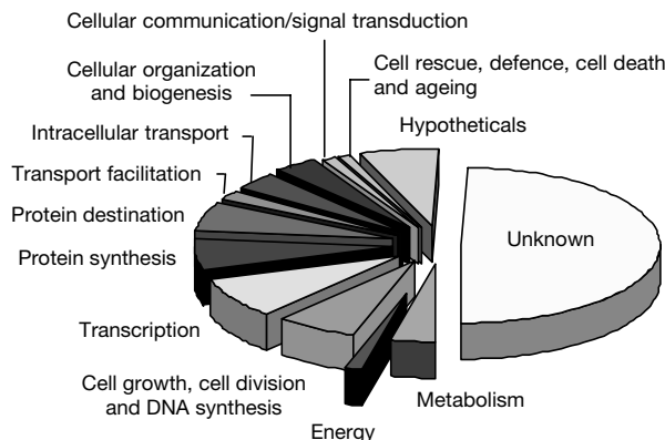
Figure 1 Distribution of predicted E. cucuruli proteins among functional groups. The corresponding gene list is given in the Supplementary Information.
