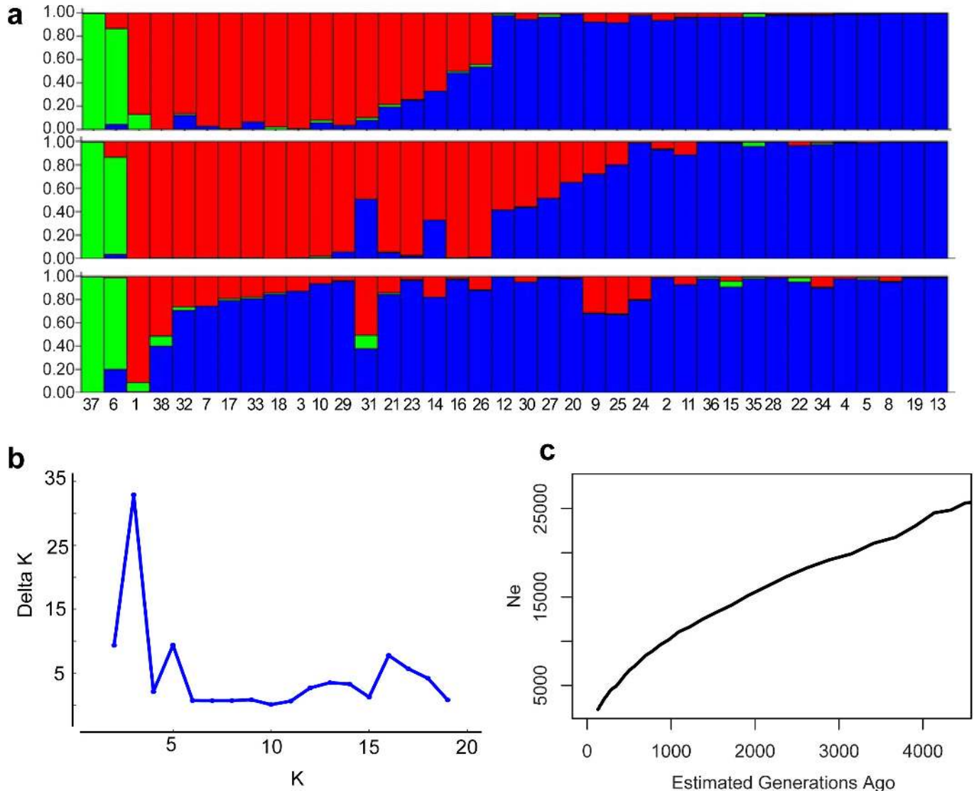
Extended Data Figure 3 | Population structure of F. excelsior in Europe. a , Results from STRUCTURE; three replicates were run for k = 3 , with each replicate using a different set of 8,955 SNPs as input. Numbers refer to samples, whose locations are given in Supplementary Table 11.
