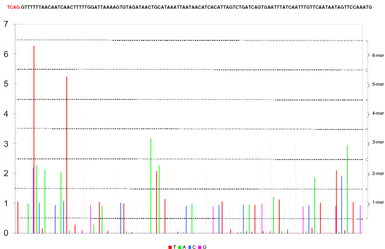
Figure 3. Flowgram of a 113 base read from an M. genitalium run.
