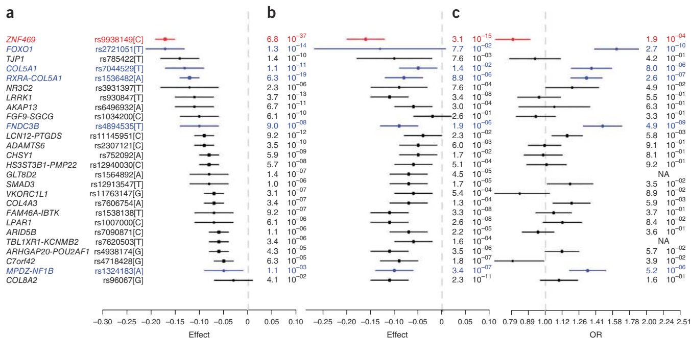
Figure 2 Association with CCT in European and Asian populations, and with keratoconus risk in European populations. (a) Association with CCT in European populations (set 1). (b) Association with CCT in Asian populations (set 2). (c) Association with keratoconus risk in European populations. This plot is a standard forest plot, but, instead of showing study-specific effects, it shows the association effects in the three panels for each locus. The allele is chosen as the CCT-reducing allele (boxes that represent the point estimates in a and b are on the left side of the dashed line, effect on CCT < 0). Effect on CCT is in standardized units. Given the association between reduced CCT and elevated keratoconus risk, for the effect directions to be consistent, the CCT-reducing allele would be the keratoconus risk allele (boxes that represent the OR of keratoconus in c on the right side of the dashed line, OR > 1). Five loci in blue, FOXO1 , two SNPs at COL5A1 , FNDC3B and MPDZ-NF1B , are the CCT-associated loci that are significantly associated with keratoconus risk after correction for multiple testing and also show consistent effect directions. The ZNF469 locus is marked in red because the CCT-reducing allele is significantly associated with a lower risk of keratoconus. rs1564892 and rs7620503 were not genotyped in the keratoconus case-control studies and are therefore presented as missing values (NA).
