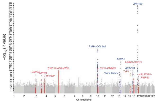
Figure 1 Manhattan plot of set 1 meta-analysis results. Association results ( -\log_{10} P values) are plotted for each chromosome. A blue dot and the corresponding gene name indicate that the locus is known in European populations. The red dot and the corresponding gene name indicate that the locus has not previously been reported as associated with CCT in European populations.
