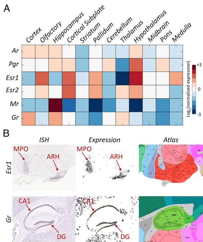
Fig. 1. Expression of steroid receptors in the mouse brain. (A) Expression of six steroid receptors across the 12 brain regions. Reported values are the average expression energy per region normalized to the average expression across the whole brain and then \log_2 -transformed. (B) Example sagittal sections from the Allen Brain Atlas (4) showing the ISH (Left), expression mask (Middle), and corresponding atlas section (Right) of Esr1 in the HY (Top) and Gr in the hippocampus (Bottom). Red arrows indicate the MPO, ARH, CA1, and DG.
