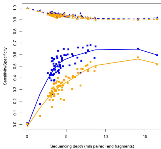
Figure 3. MethylCap-seq sensitivity reaches a plateau phase for increasing sequencing depths.
