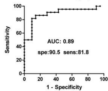
E) ROC of LDA (UK)
