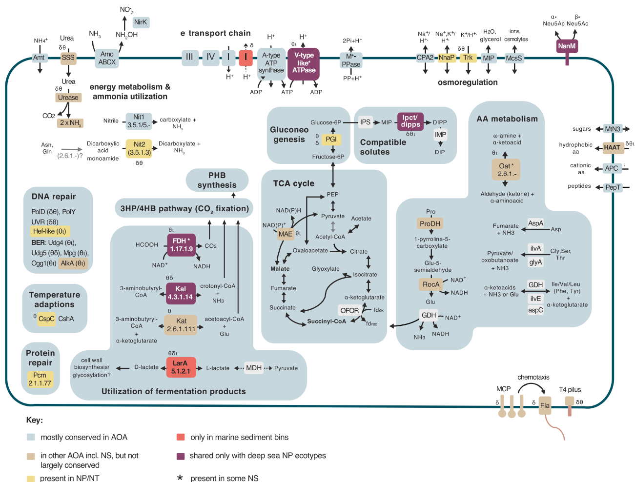
Fig. 5 Metabolic reconstruction of amoA -NP-theta, amoA -NP-delta, and amoA -NP-iota AOA. Schematic reconstruction of the predicted metabolic modules in the sediment MAGs, as discussed in the text. Color code of enzymes/complexes indicates conservation status in AOA. Unless specified by greek letters ( \theta\delta\iota ), enzymes/modules are present in all sediment clades. Dashed lines indicate hypothetical reactions. The gray arrow indicates an alternative OFOR reaction. Complexes of the electron transport chain are labeled with roman numerals. Transporters are named according to TCDB classification. Enzymes, gene accession numbers, and transporter classes are also listed in Supplementary Tables 2 and 4. Amo ammonia monooxygenase, NirK nitrite reductase, Nit1 nitrilase, Nit2 nitrilase/omega-amidase, AA amino acid, Fdh formate dehydrogenase, Kal 3-aminobutyryl-CoA ammonia lyase, Kat putative 3-aminobutyryl-CoA aminotransferase, LarA lactate racemase, Pcm protein-L-isoaspartate carboxylmethyltransferase, MCP methyl-accepting chemotaxis protein, Fla archaeallum, PolD polymerase family D, PolY translesion polymerase family Y, UVR excision repair system, Hef-like Hef/FANCM/Mph1-like helicase, BER base-excision
