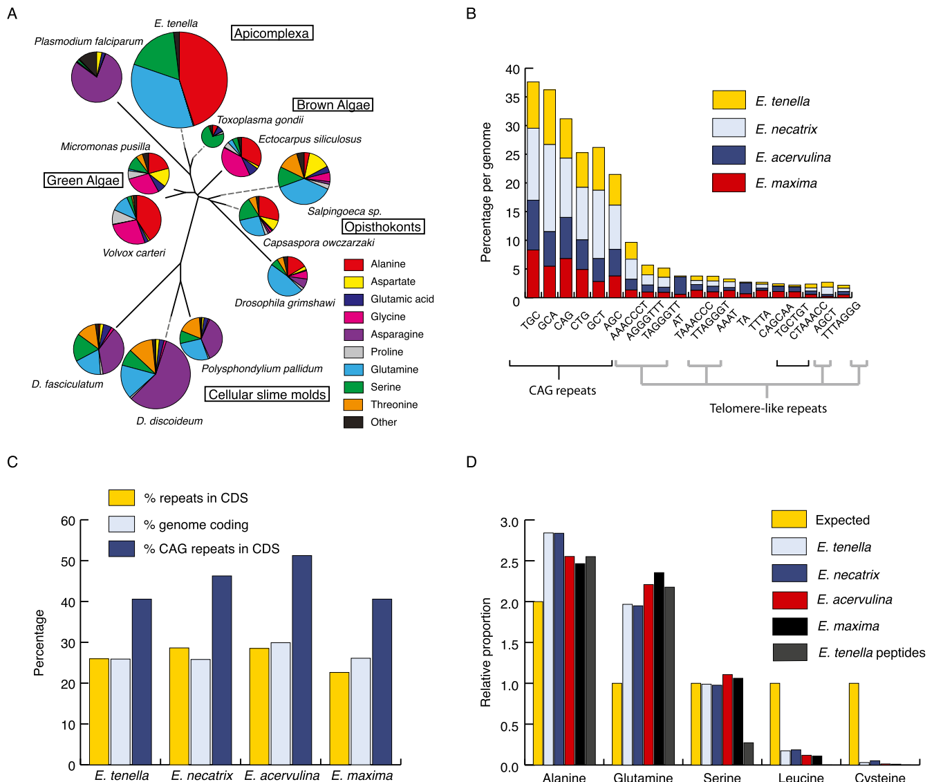
Figure 2. Characterization of HAARs in Eimeria protein sequences. (A) Eimeria tenella has a greater number of HAARs than any other genome sequenced and a distinct distribution of HAAR types compared with other repeat-rich genomes, including Plasmodium falciparum and the more closely related and not especially repeat-rich Toxoplasma . (B) The most common STRs in Eimeria genomes are variations on CAG. The second most common are variations on a telomere repeat which we call telomere-like repeats due to their locations throughout the genome. (C) CAG repeats occur in protein-coding regions of the genome more than expected. (D) CAG repeats can encode strings of one of five amino acids. In Eimeria they tend to encode alanine and glutamine more often than expected, serine as often as expected, and leucine and cysteine more rarely than expected. A very similar pattern is observed in a limited selection of E. tenella peptides derived from proteomics experiments.
