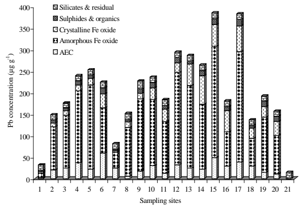
Fig. 5: Geochemical distribution of Pb concentration ( \mu\text{g g}^{-1} ) in sediment samples at different sampling sites of the study area
