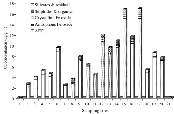
Fig. 2: Geochemical distribution of Cd concentration ( \mu\text{g g}^{-1} ) in sediment samples at different sampling sites of the study area
