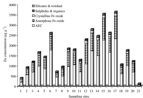
Fig. 6: Geochemical distribution of Zn concentration ( \mu\text{g g}^{-1} ) in sediment samples at different sampling sites of the study area
