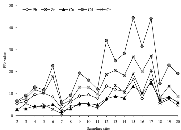
Fig. 7: Enrichment factors (EFc) of trace metals in sediment samples at different sampling sites of the study area
