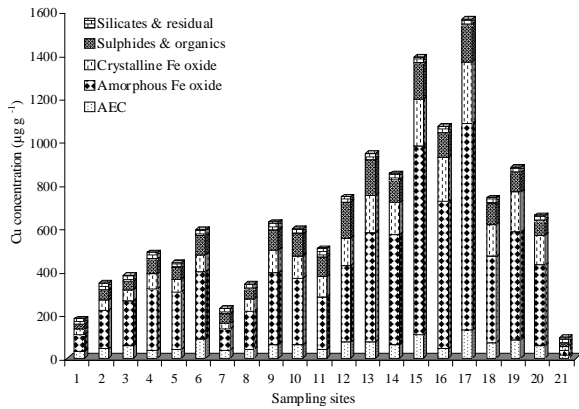
Fig. 3: Geochemical distribution of Cu concentration ( \mu\text{g g}^{-1} ) in sediment samples at different sampling sites of the study area
