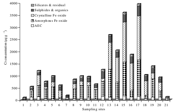
Fig. 4: Geochemical distribution of Cr concentration ( \mu\text{g g}^{-1} ) in sediment samples at different sampling sites of the study area
