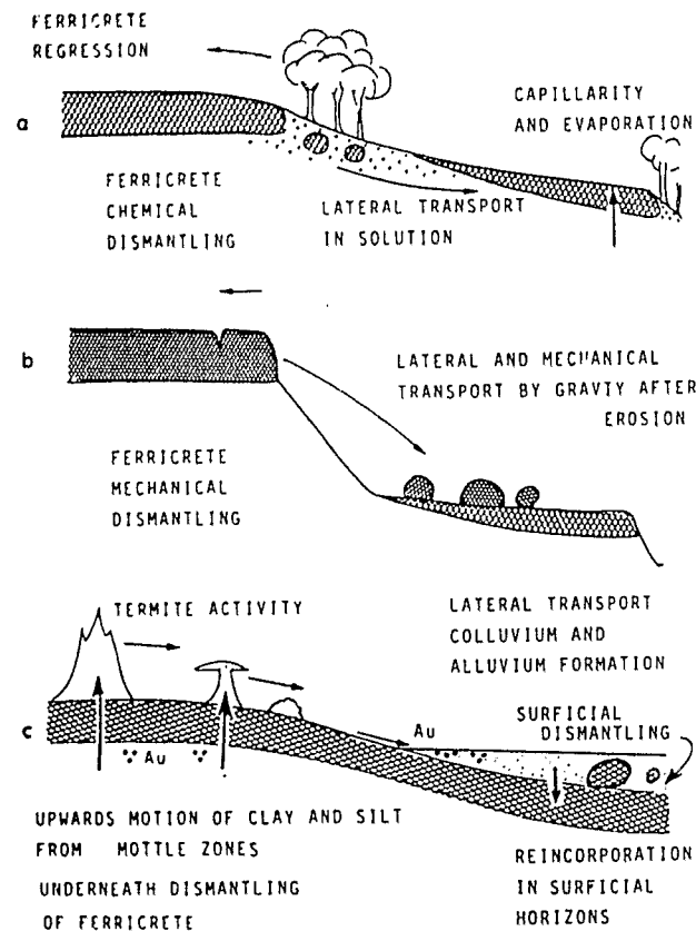
Fig. 16.6. Lateral movements of material in landscapes; a. lateral migration of iron in solution; b. lateral mechanical movements of disaggregated blocs of ferricretes; c. lateral transport of material reworked by termite activity.
