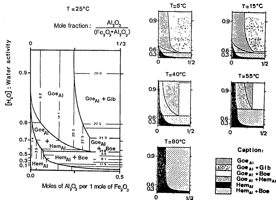
Fig. 16.11. Stability diagrams for Al-goethite, Al-hematite, gibbsite and boehmite at 25°C and at different temperatures as a function of water activity (from Trolard and Tardy, 1987).
