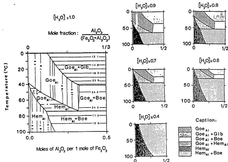
Fig. 16.12. Stability diagrams for Al-goethite, Al-hematite, gibbsite and boehmite at [H_2O] = 1 and at different activity of water, as function of temperature (from Trolard and Tardy, 1987).
