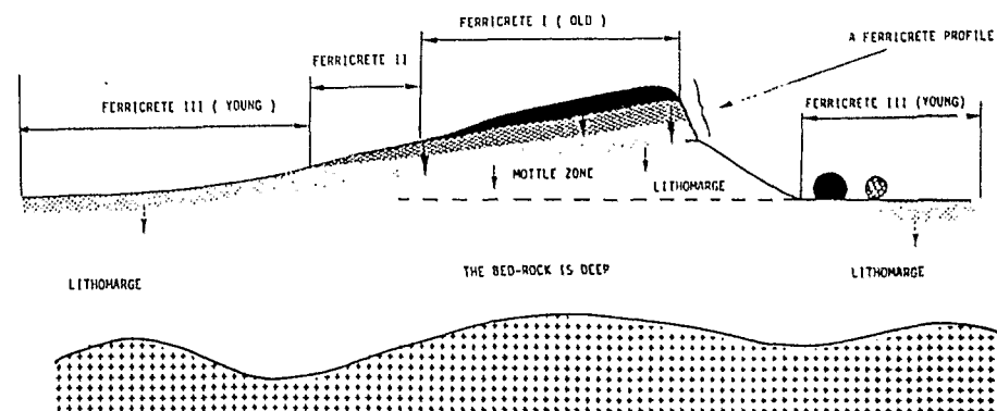
Fig. 16.2. Lateral distribution of lateritic facies in a tropical landscape shaped by erosion and subsequent alteration.
