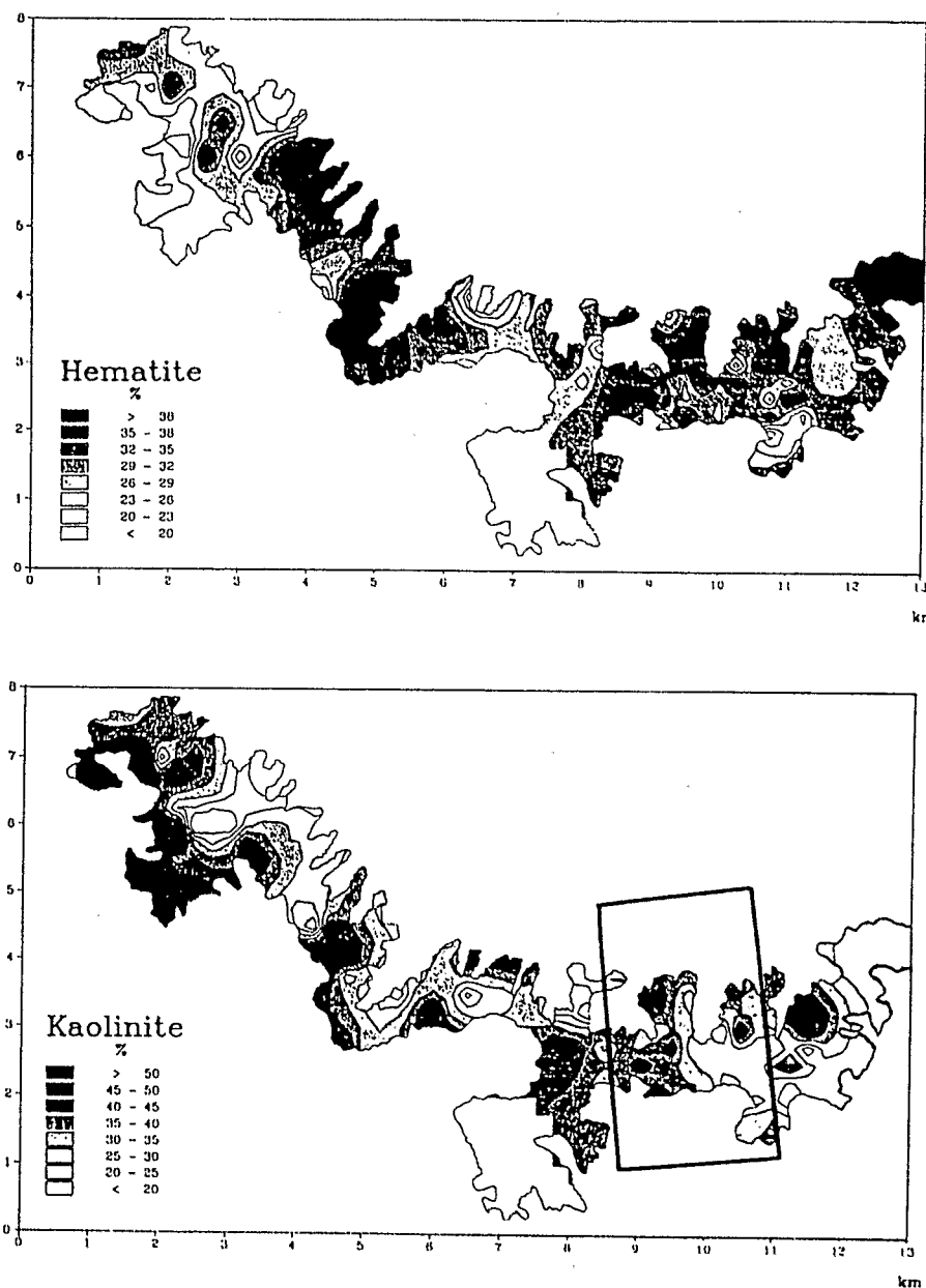
Fig. 16.3. Patchworks of different petrographical, mineralogical and geochemical facies of ferricrete, due to differential erosion over a given morphological surface. The soil surface was permanently submitted to a contrasted tropical climate and outcropping ferricretes are of different ages and degrees of evolution (Mazaltarim, 1989; Boeglin, 1990; Freyssinet, 1990).
