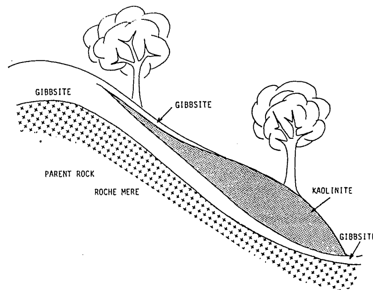
Fig. 16.9. Distribution of gibbsite and kaolinite in lateritic profiles of the Ivory Coast, showing: a. only gibbsite; b. a succession of gibbsite-kaolinite-gibbsite; and c. a succession of kaolinite-gibbsite from top to bottom of the profiles and from upslope to downslope on the landscapes (after Delvigne, 1965).
