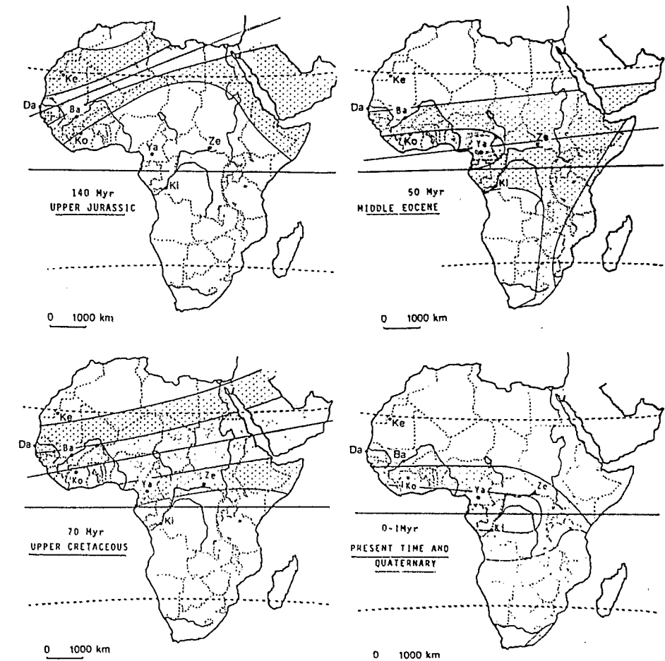
Fig. 16.13. Paleoclimatic potential distribution of bauxites (dark shadowed) in equatorial domains of ferricretes (light shadowed) in contrasted tropical zones of Africa (from Parrish et al., 1982, and after Kobilsck, 1989).
