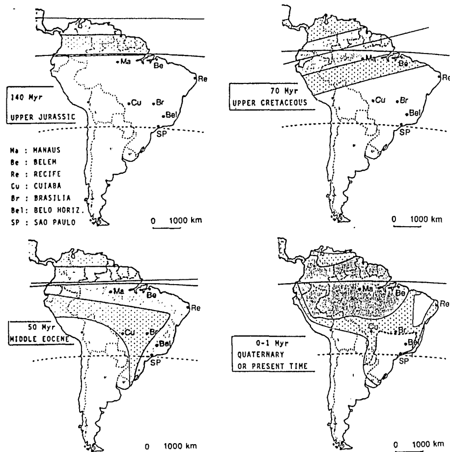
Fig. 16.14. Paleoclimatic potential distribution of bauxites (dark shadowed) in equatorial domains of ferricretes (light shadowed) in contrasted tropical zones of South-America (from Parrish et al., 1982, and after Kobilsck, 1989).
