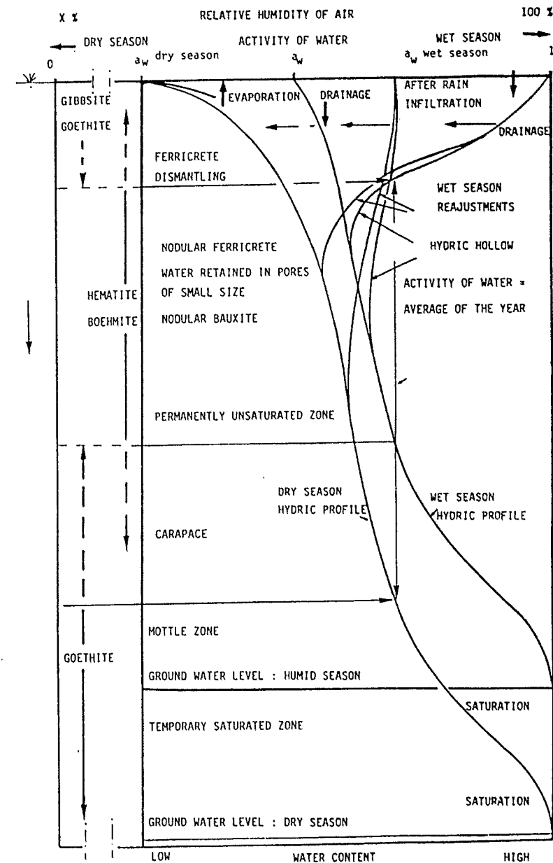
Fig. 16.10. Seasonal distribution of water activity across a weathering profile, in a non-equilibrium situation, above a deep ground water level (10 m) (after Tardy et al., 1988a).
