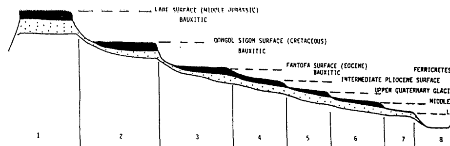
Fig. 16.1. The seven peneplanation surfaces of Michel (1973) capped by laterites of different kinds (bauxites or ferricretes) and of different degree of evolution, observable from the Fouta Djallon in Guinea to the Niger alluvial plain in Mali.
