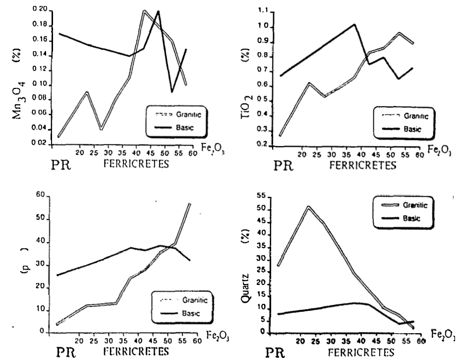
Fig. 16.5. An example of the mineralogical and chemical composition of ferricretes of Gaoua (Burkina Faso), located on different basic or granitic parent rocks (PR). For low \text{Fe}_2\text{O}_3 contents, compositions are distinct: ferricretes are lithodependent. For high \text{Fe}_2\text{O}_3 contents, compositions are homogenized: ferricretes seem to be litho-independent. (From Tardy et al., 1988.)
