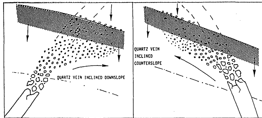
Fig. 16.7. Formation of geochemical halos around mineralized quartz veins. Vertical lowering of the soil surface, deepening of the weathering front and apparent lateral motion of material upslope or downslope. (Adapted from Leprun, 1979.)
