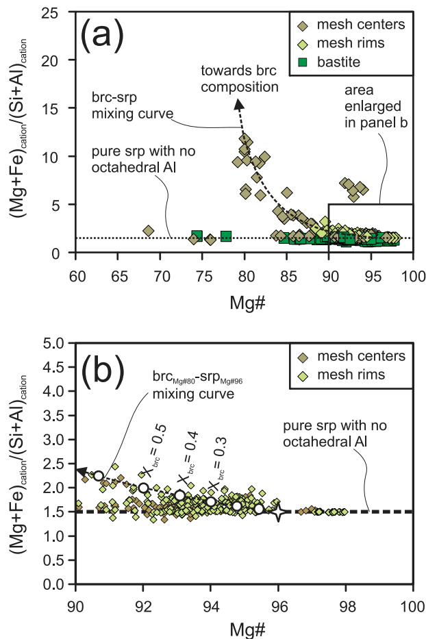
Fig. 6. Plot of [(\text{Mg} + \text{Fe})/(\text{Si} + \text{Al})]_{\text{cation}} vs Mg-number of pseudomorphic serpentine \pm brucite. (a) The entire compositional range found in the studied serpentinites. Mesh center and rim compositions lie close to the mixing curve between serpentine, [(\text{Mg} + \text{Fe})/(\text{Si} + \text{Al})]_{\text{cation}} \sim 1.5 , Mg-number > \sim 90 , and brucite [(\text{Mg} + \text{Fe})/(\text{Si} + \text{Al})]_{\text{cation}} \gg 25 , Mg-number \sim 80 . (b) The compositional range corresponding to Mg-number between 90 and 100 and [(\text{Mg} + \text{Fe})/(\text{Si} + \text{Al})]_{\text{cation}} of 0–5. For the sake of clarity, bastite compositions are omitted. Assuming Mg-number = 80 brucite as one end-member and Al-free, Mg-number = 96 serpentine as another (white star, chosen as an end-member composition because the vast majority of analyses have lower Mg-number), we estimated the amount of brucite in the mixed analyses (white dots with the molar fraction of brucite, X_{\text{brc}} , in the mixture). All iron is regarded as \text{Fe}^{2+} . This calculation maximizes brucite contents, which in reality are probably lower.
