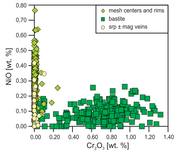
Fig. 7. NiO vs \text{Cr}_2\text{O}_3 contents (wt %) of pseudomorphic serpentine \pm brucite and serpentine \pm magnetite veins. Pseudomorphic replacements after olivine (mesh centers and rims) and orthopyroxene (bastite) are easily distinguishable, suggesting limited mobility of Ni and Cr during serpentinization.
