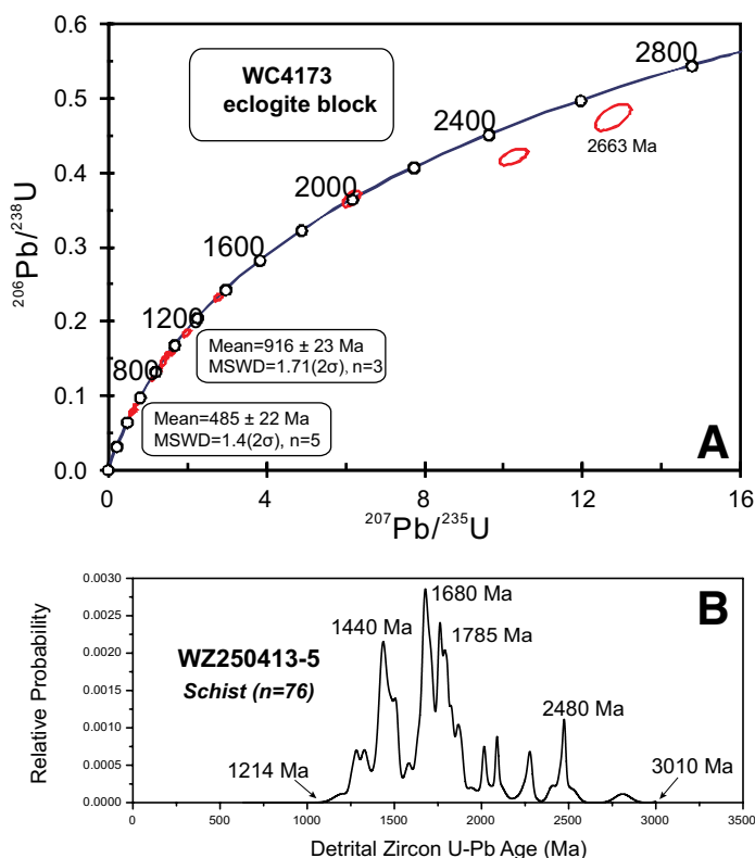
Figure 9. (A) Zircon concordia diagrams showing results for the eclogite sample (WC4173). MSWD—mean square of weighted deviates. (B) Relative probability plot of zircon U-Pb ages (Ma) for the schist sample WZ250413-5 from the central Qilian Shan.
