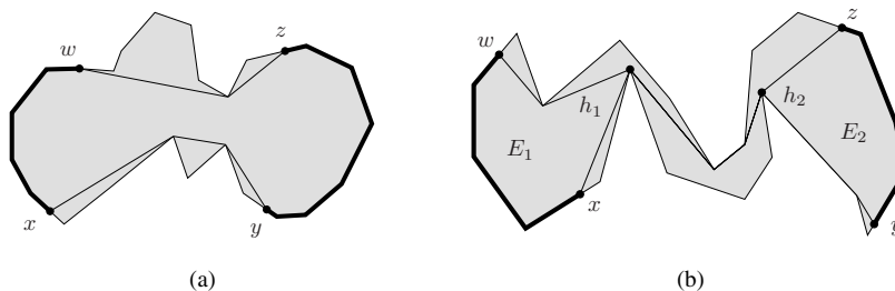
Fig. 5. Two funnels: (a) a fat funnel and (b) a skinny funnel.
