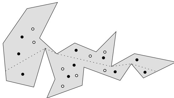
Fig. 1. A ham-sandwich geodesic with r = 8 and b = 10 .
