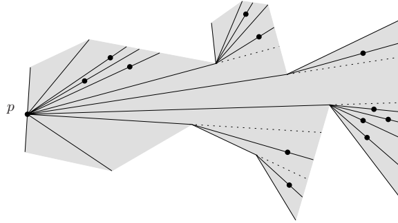
Fig. 4. Computing a tree that contains a geodesic from p through every point of B' .
