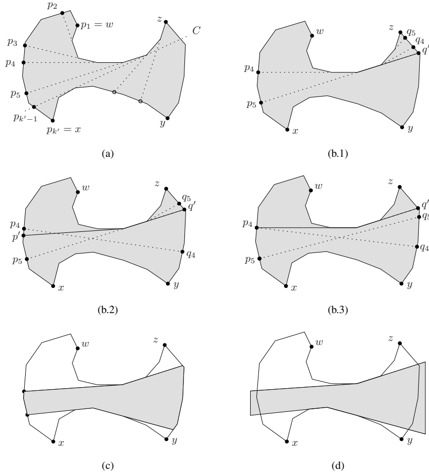
Fig. 6. Reducing a fat funnel to a 6-gon by (a) extending the upper chain edges until they intersect [wx] , (b.1)–(b.3) using p_i and p_{i+1} to eliminate all but one reflex vertex of the upper chain, and (c)–(d) replacing the two convex chains with vertical edges.
