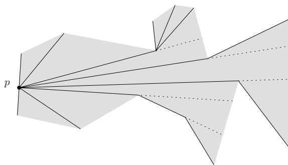
Fig. 3. The augmented shortest path partition for a point p . Edges added during the augmenting step are dotted.
