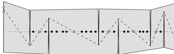
Fig. 8. The lower bound input to a ham-sandwich algorithm.
